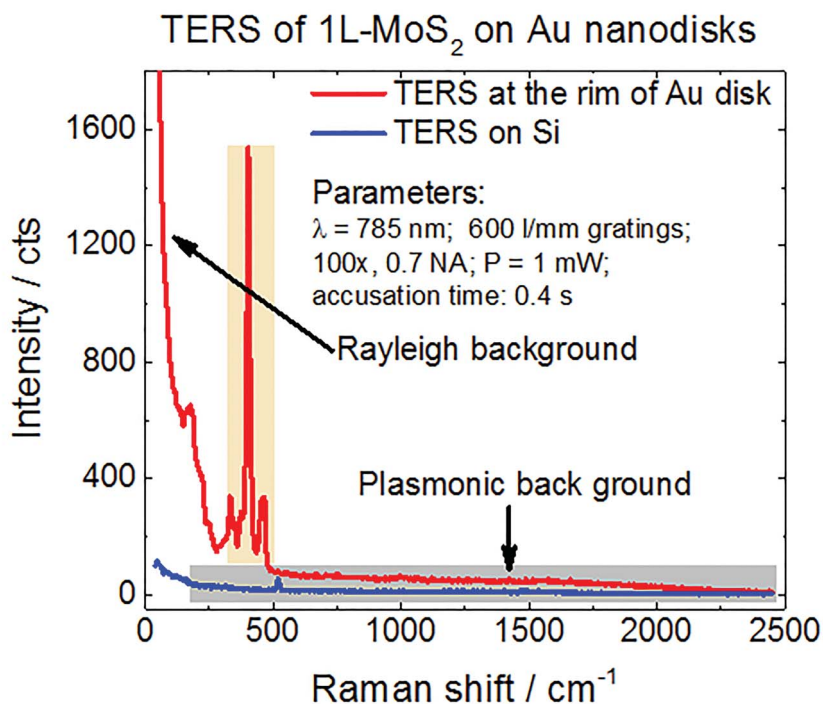
Fig. 1 Typical as measured TERS spectra taken at the edge of the Au disk and on Si.
