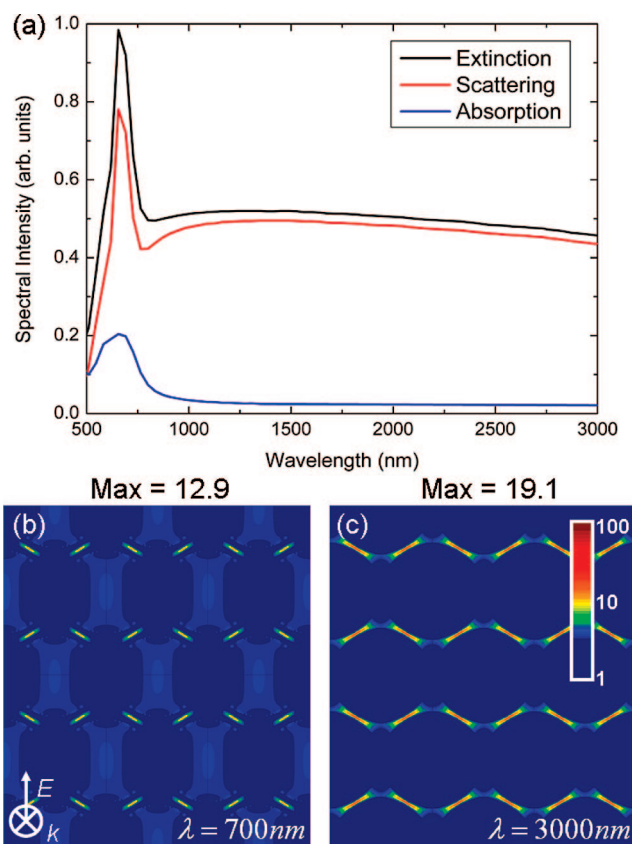
Figure 2. FDTD simulation results for an HCP Au nanoshell array. The geometry of the nanoshell is (r_1, r_2) = (150, 172) nm, the separation is d = 8 nm, and the grid size is 2 nm. The periodic unit cell is composed of four half-nanoshells. Panel a shows the extinction (black), scattering (red), and absorption (blue). Panels b,c show the local electromagnetic field enhancements at wavelengths of 700 and 3000 nm, respectively.
