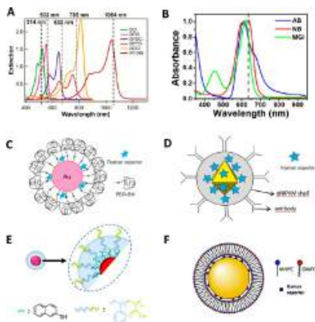
Figure 20. (A, B) Resonant Raman configuration; multiple-dye conjugates capable of producing signals over a wide range of common excitation wavelengths (A) and dye conjugates with similar optical properties for multiplexing (B). Adapted with permission from refs 335 and 359. Copyrights 2014 American Chemical Society and 2015 Wiley-VCH, respectively. (C–F) Configuration for protection and stabilization; thiolated polystyrene (C), poly( N -isopropylacrylamide) shell (D), PSS–PAA block copolymer encapsulation (E) and phospholipid-coated surface-enhanced Raman scattering nanotags (F). Adapted with permission from refs 351, 359, 367, and 363. Copyrights 2007 Springer-Nature, 2015 Wiley-VCH, 2018 Royal Society of Chemistry, and 2010 American Chemical Society, respectively.
