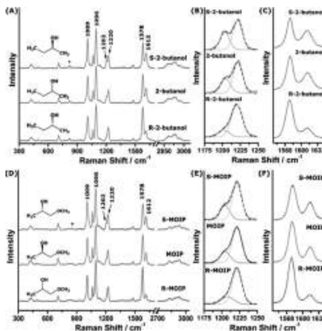
Figure 23. (A, D) Normalized SERS spectra of the MPY–Ag complex separately immersed in different chiral alcohols (2-butanol and MOP, respectively) in their optical pure and racemic forms. (B, E) and (C, F) Magnifications of the 1175–1250 cm −1 and 1540–1650 cm −1 spectral regions of the SERS spectra shown in (A) and (D), respectively. Reproduced with permission from ref 427. Copyright 2014 Wiley-VCH.
