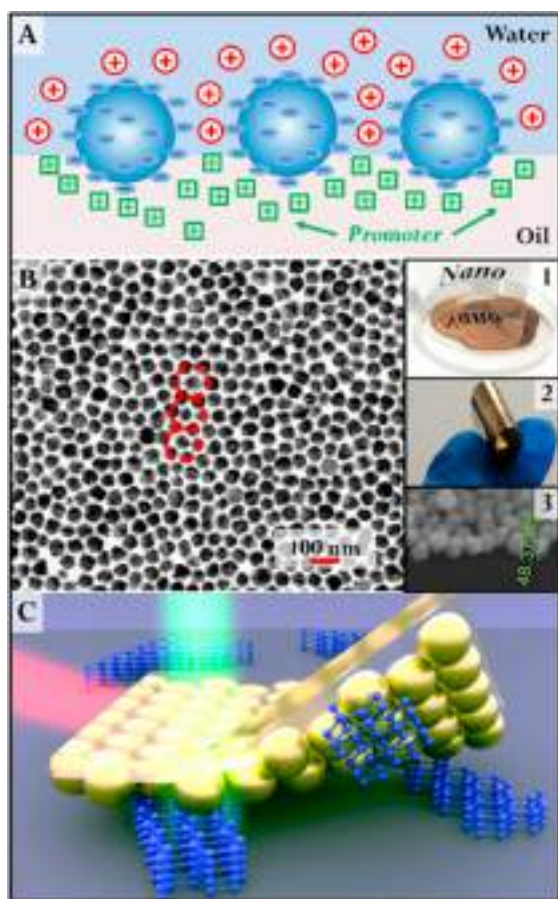
Figure 11. (A) Schematic illustration of “promoter” induced NP interfacial self-assembly. (B) SEM characterization of SENS showing short-range hexagonal particle packing. Insets 1 and 2 show optical images of a Au MeLLF and a Au SENS, respectively. Inset 3 is a tilted SEM image of SENS showing the NPs anchored in the polymer. (C) Schematic illustration of SENS used for solvent-free SERS analysis. Adapted with permission from refs 234 and 238, copyrights 2016 American Chemical Society and 2018 Elsevier B. V., respectively.
