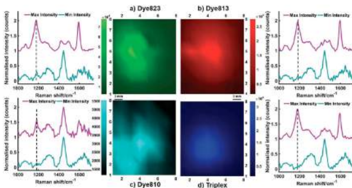
Figure 40. SESORRS false-color two-dimensional (2D) heat maps of the peak intensity at (a) 1178\text{ cm}^{-1} (dye 823), (b) 1181\text{ cm}^{-1} (dye 813), (c) 1185\text{ cm}^{-1} (dye 810) and (d) 1181\text{ cm}^{-1} (triplex). Measurements were performed using an xy translational stage in step sizes of 3\text{ mm} to create an image of 8 \times 8 pixels. 2D heat maps were generated and show the tracking of each of the four MTS models through 10\text{ mm} of tissue. Clear discrimination is seen between spectra collected at the point of maximum intensity, where the nanotags were spotted, and that collected where the nanotags were not present. The corresponding maximum and minimum collected 8\text{ mm} offset spectra also confirm the presence of the nanotags in regions where the MTS were spotted (a–d). Reproduced with permission from ref 760. Copyright 2018 Royal Society of Chemistry.
