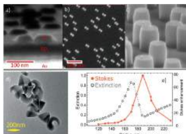
Figure 16. Resonant nanostructures fabricated through HCL. (a) Side view of SERS substrate consisting of gold nanodisk dimers fabricated on top of a Au mirror with a \text{SiO}_2 spacer layer in between; (b) top view of a Au dimer-on-mirror SERS substrate illustrating the uniform dimensions and orientations of the individual nanostructures. (c) Si nanopillars and (d) chiral Si colloids fabricated by a variant of HCL; (e) illustration of near-field amplification and Raman scattering enhancement in Si nanodisks supporting an anapole resonance. Reproduced with permission from refs 281–283 and 285. Copyrights 2015 Royal Society of Chemistry, 2017 American Chemical Society, 2017 Wiley-VCH, and 2018 American Chemical Society, respectively.
