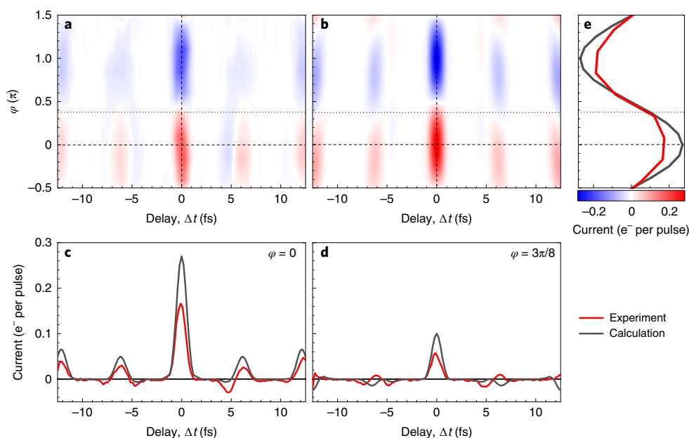
Fig. 2 | Interferometric current autocorrelations dependent on the CEP of the driving pulses. a, b , Colour map of the measured (a) and calculated (b) 2D interferometric autocorrelation acquired as a function of temporal delay \Delta t and phase \varphi of the sinusoidal current modulation. c , Interferometric autocorrelation (red line) of two identical single-cycle pulses with CEP set to deliver the maximum peak current using the current driven at the nanogap as a nonlinear signal (dashed line in a, b). The extreme order of nonlinearity is underlined by the absence of signal when the maxima of the field do not overlap at the periodicity of the carrier wavelength. The width of the central peak is \sim 1 fs. The experimental data are compared with the equivalent trace derived from the calculations (black line). d , Same as c but acquired at \varphi = 3\pi/8 (dotted line in a, b). e , Vertical cut of the 2D colour map at \Delta t = 0 , which is equivalent to a single pulse illuminating the nanogap. The sinusoidal modulation of the current with phase \varphi is shown for the experiment (red line) and theory (black line).
