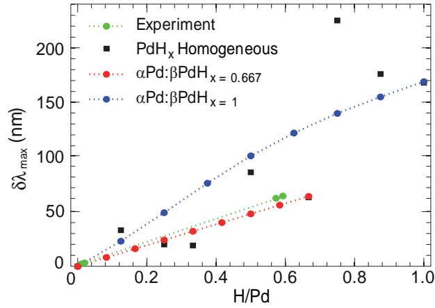
Figure 5: LSPR shifts calculated for a Pd-H disk of 20 nm thickness and 300 nm diameter plotted as a function of z = \text{H/Pd} ratio. The resonance shifts are calculated using Bruggeman's effective dielectric function (Eq.(2)) with the \beta phase taken as \text{PdH}_{x=0.667} (red dots), and as \text{PdH}_{x=1} (blue dots). A comparison with experimental results from Ref. 6 (green dots) is shown.
