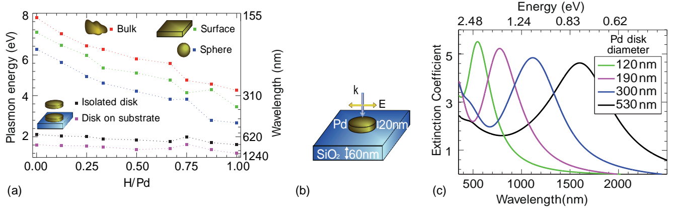
Figure 2: (a) Plasmonic resonance energies of the \text{PdH}_x systems for (i) bulk, (ii) surface, (iii) dipolar LSPR in a spherical particle in the electrostatic limit, (iv) isolated disk of 20 nm thick and 190 nm diameter and (v) the same disk deposited on \text{SiO}_2 substrate, obtained with use of dielectric functions calculated through the TDDFT as a function of x=H/\text{Pd} ratio. The dotted lines are guides to the eye. (b) Schematics of the system used in the BEM calculations to obtain the far-field optical response of the \text{PdH}_x nanodisks. Disks of thickness 20 nm and different diameters and deposited on a 60 nm thick \text{SiO}_2 substrate and illuminated by a polarized planewave incident normally from the top. (c) Extinction spectra calculated using the ab initio dielectric function for Pd disks of 20 nm thickness for different diameters.
