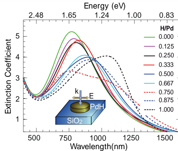
Figure 3: Extinction spectra of \text{PdH}_x disks of 20 nm thickness and 190 nm diameter with uniform stoichiometry placed on \text{SiO}_2 substrate evaluated for different x=H/\text{Pd} values. The disks are characterized by the dielectric functions as obtained from the TDDFT calculations in Fig. 1(b).
