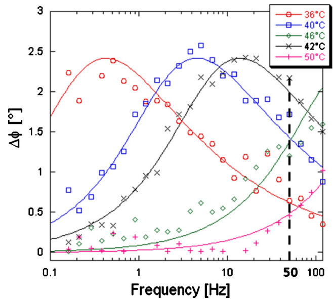
FIG. 2. (Color online) Phase shift measured as a function of the frequency over an island of PVAc. Statistical error is 0.25 for f > 1 Hz and 0.35 for f \leq 1 Hz. Lines are fits derived from a KWW model with amplitude and shape parameters fixed for all curves. The dashed line indicates the imaging frequency of Fig. 3.
