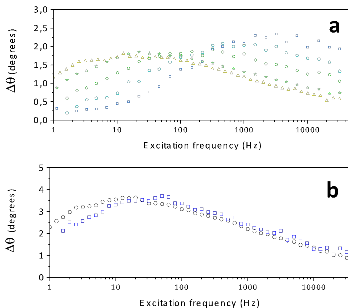
FIGURE 2. AFM based dielectric loss spectra for the \beta relaxation of PMMA. (a) Spectra obtained at 313, 323, 333, 343 and 353 K (from left to right) with a SCM PIT probe. (b) Spectra obtained with a NN-HAR-FM60 probe at 313 and 323 K.
