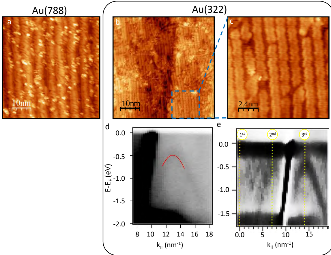
Figure 9.6: ARPES characterization of VB on Au(322). (a-c) STM images of (3,1)-chGNRs grown (a) on Au(788) (50 x 50 nm, V_s = 1.0 V, I_t = 50 pA) and (b,c) on (Au(322) (50 x 50 nm, 10 nm x 10 nm, V_s = -0.2 V, I_t = 20 pA). (d) Raw signal and (e) second derivative of the photoemission intensity reflecting the valence band dispersion.
