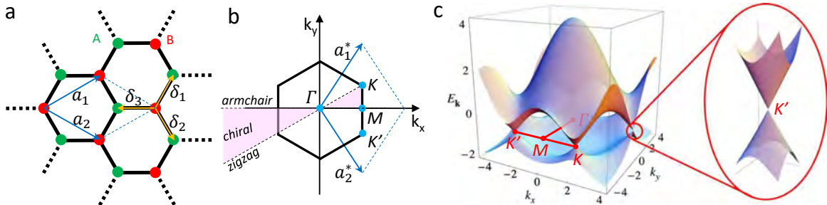
Figure 3.1: (a) Lattice structure of graphene including its primitive \mathbf{a}_i (blue arrows) and translation \delta_i vectors (yellow arrows). (b) Corresponding Brillouin zone in the reciprocal lattice including reciprocal vectors \mathbf{a}_i^* (blue arrows). (c) Electronic band structure calculated using an orthogonal tight-binding model and considering only nearest neighbor atom interactions. The inset depicts the conical energy band dispersion of one Dirac point near the Fermi energy (adapted from 8 ).
