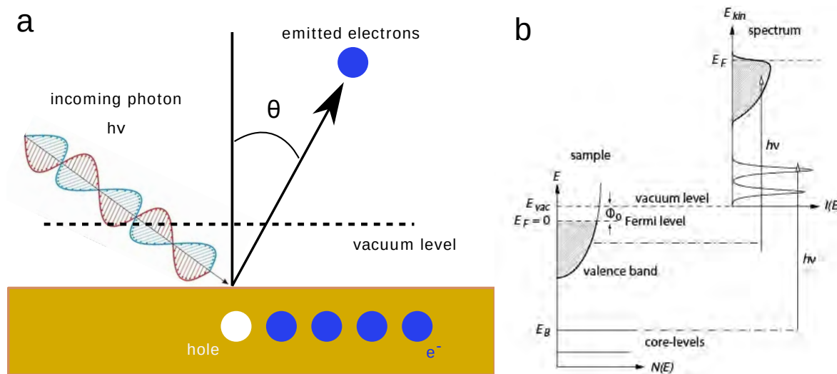
Figure 2.13: Photoemission models. (a) Photoelectric effect and (b) three step model describing the path followed by the photo ejected electron until it escapes from the surface. Copied from ref. 228
