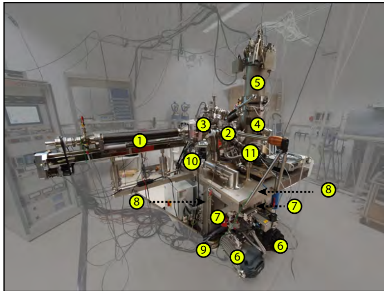
Figure 2.10: Commercial ‘Apollo’ LT-STM equipment employed in this thesis. Located at Materials Physics Center research center. Numbered circles correspond to (1) manipulator, (2) load-lock, (3) preparation and (4) microscope chambers; (5) cryostates; (6) scroll, (7) turbo and (8) ion pumps (inside the metallic); (9) pneumatic dumping legs, (10) mass spectrometer and (11) molecular evaporators.
