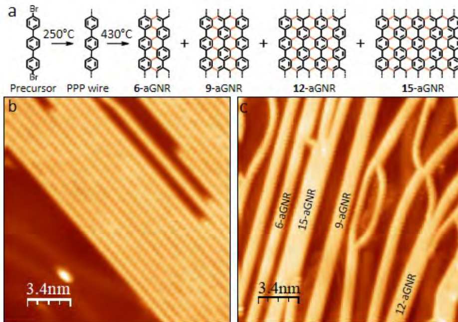
Figure 4.1: (a) Schematic synthesis from DBTP molecular precursor on Au(111). STM topography images of (b) PPP nanowires (24.6 nm 2 , I_t = 0.22 nA, V_s = 1.0 V) and (c) a-GNRs (24.6 nm 2 , I_t = 0.22 nA, V_s = -1.7 V), where text inlets indicate the different widths of aGNRs
