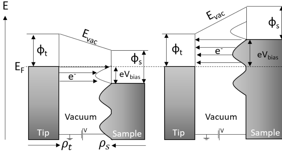
Figure 2.3: Model illustrating the dependence of the probed sample states on the voltage polarity, being the voltage applied on the sample.
