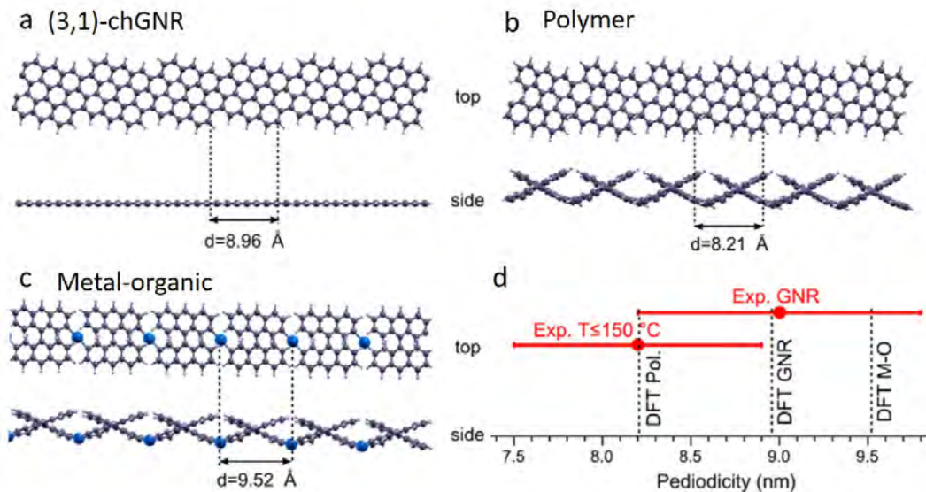
Figure 6.4: Relaxed structures for (a) free-standing (3,1)-GNRs, (b) poly-2, and (c) metal-organic chains. (d) Comparison of the periodicities of the calculated structures with those measured experimentally for the GNRs and for the nonplanar structure on Ag(111). The latter fits the polymer period, and its error margin (shown as the standard deviation) is well below the periodicity of the metal-organic chain.
