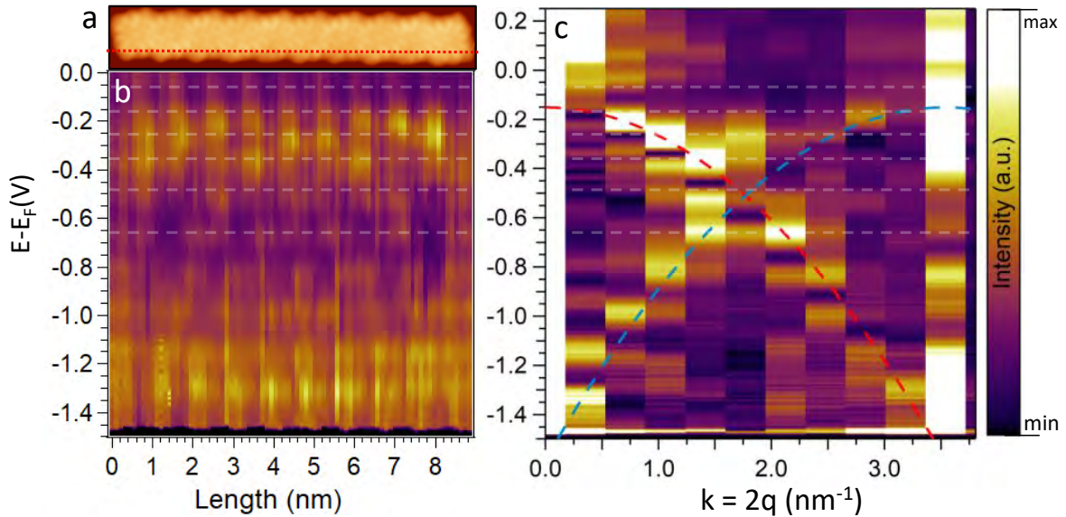
Figure 9.4: Valence band dispersion by FT-STs. (a) Constant-current STM image of the same ribbon than in Figure 9.3, showing the path (red dashed line) followed by the equidistant dI/dV spectra. (b) Color-coded conductance signal obtained from equidistant dI/dV point spectra (open-feedback parameters: V_s = 1.50 V; I_t = 0.8 nA; V_{rms} = 12 mV) on the ribbon and along the red dashed line displayed in panel g. (c) Line-by-line Fourier transform from the stacked spectra in panel (b), showing the two-parameter parabolic fit (red dashed line) used for extracting the effective mass. The additional parabola centered around the Brillouin zone edge is displayed with a green dashed line. Gray horizontal lines corresponding to the voltage biases of maps in Figure 9.3a-f are superimposed in panels (b) and (c) as a guide to the eye.
