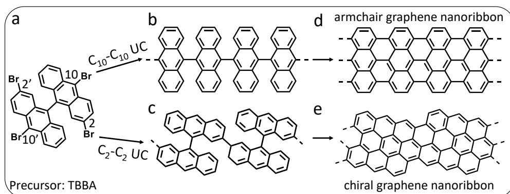
Figure 7.1: Possible synthetic routes expected from (a) TBBA precursor. (b) Debromination and C 10 -C 10 UC followed by CDH leads to (d) aGNRs formation. (c) Debromination and C 2 -C 2 UC leads to (e) chiral GNRs formation. Note that primed position x' is chemically equivalent to the corresponding unprimed position x and either would yield the same GNR.
