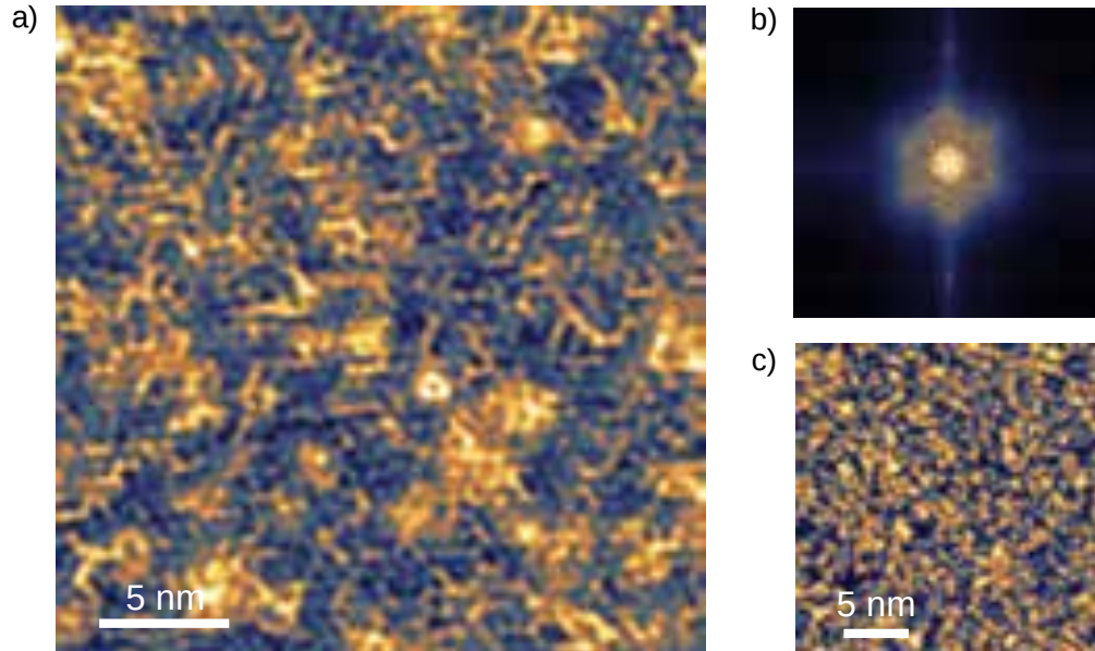
Figure 4.1.7: Striped substitutional Mo arrangement. a) STM image of the Nb 0.8 Mo 0.2 Se 2 monolayer showing stripes of Mo atoms ( V_s = +2 V, I_t = 0.15 nA, T = 4.2 K). b) FFT image of the topography in a) showing the six-fold angular stripe arrangement. c) STM image of the same region as in a) taken at the opposite polarity (occupied states) ( V_s = -0.4 V, I_t = 0.15 nA, T = 4.2 K).
