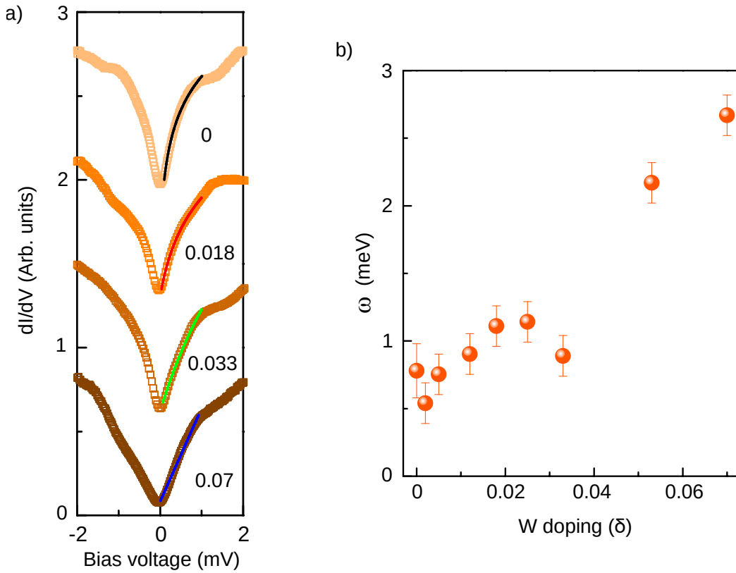
Figure 4.2.6: Electronic characterization of the observed gap in the metallic state of Ta 1- \delta W \delta Se 2 alloy. a) DOS evolution of the dip feature within \pm 1 meV in Ta 1- \delta W \delta Se 2 monolayer from \delta = 0 (pristine TaSe 2 ) up to \delta = 0.07 . All the dI/dV spectra were taken in the non-SC regime. b) Width of the dI/dV curves as a function of the W doping ( \delta ).
