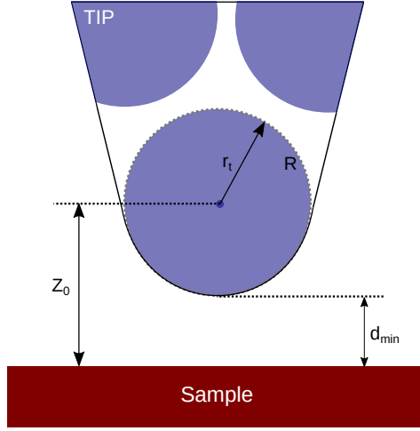
Figure 2.2.3: STM tip in the Tersoff-Hamann approximation. The tip with a single atom at its apex is assumed as a spherical object with radius r_t and curvature R . Reproduced from [109].
