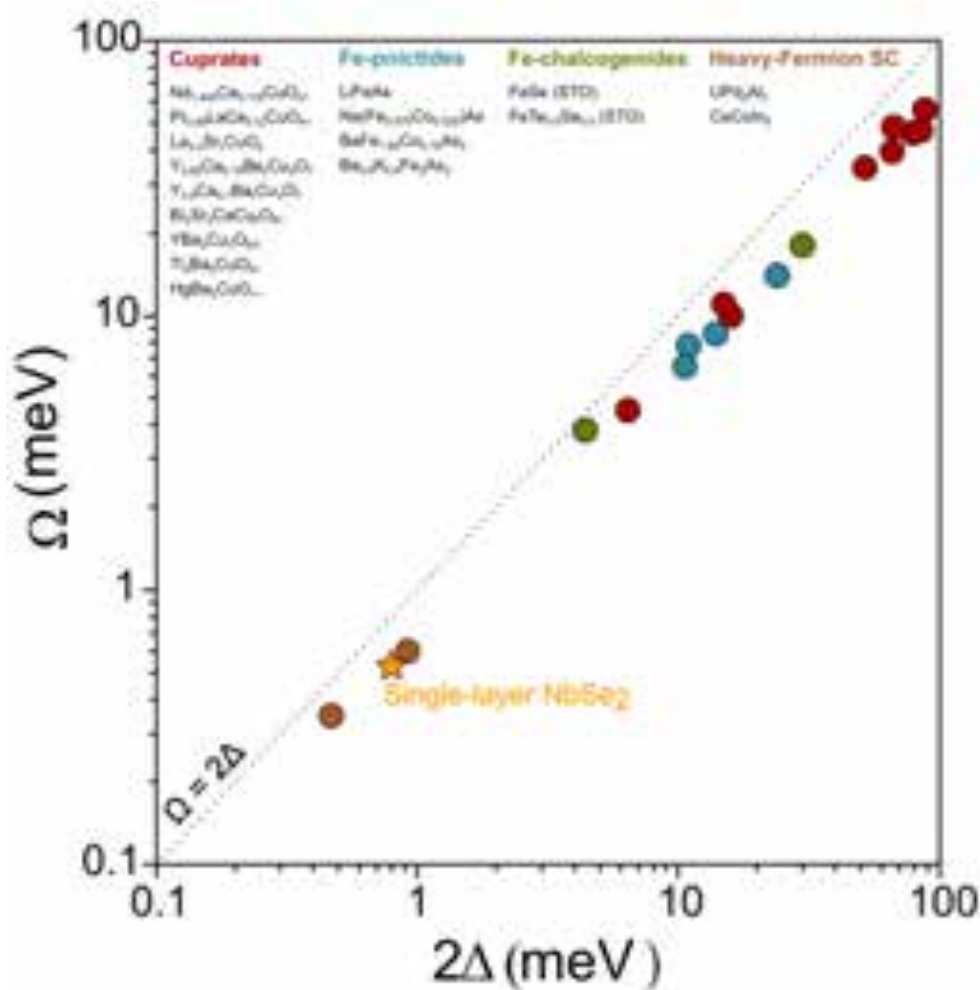
Figure 3.3.12: Universal relationship between \Omega and \Delta in unconventional superconductors.
