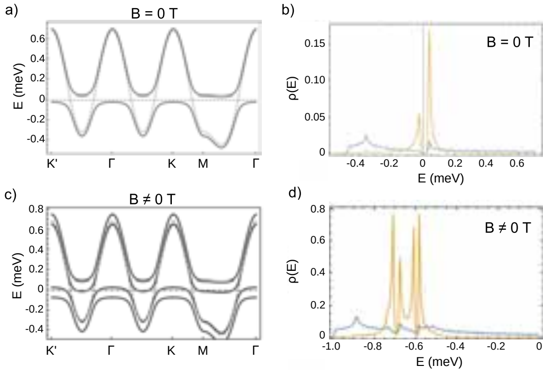
Figure 5.2.7: Theoretical gap evolution as a function of the magnetic field for a Kondo insulator. a) Opening of a bandgap as a result of the interacting c- and f-band (dashed lines). b) The corresponding DOS shows two peaks (gap) around E_F . c) In the presence of a magnetic field, the spin degenerate bands split, d) which results in four peaks in the DOS. (Calculations by Fernando de Juan (DIPC))
