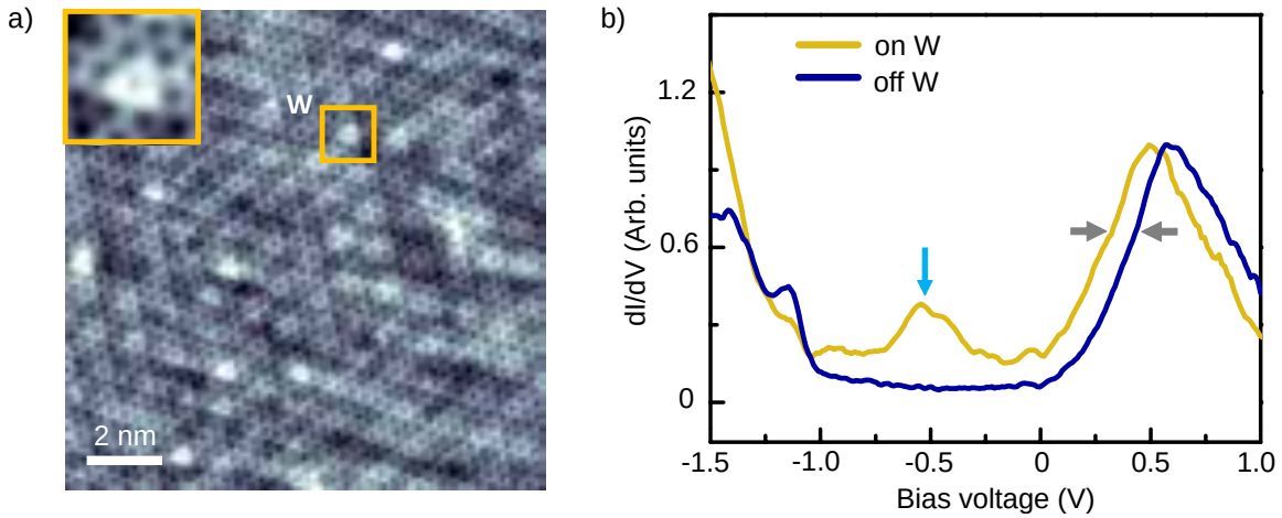
Figure 4.2.1: Identification of W impurities in SL-Ta 1- \delta W \delta Se 2 alloy. a) Atomically resolved STM image of Ta 0.994 W 0.006 Se 2 ( V_t = -1 V, I = 0.8 nA, T = 4.2 K). The inset shows a zoom-in of the W atom boxed in the main image. b) Large-scale dI/dV curves on pristine TaSe 2 (blue) and on one of the W atoms (yellow).
