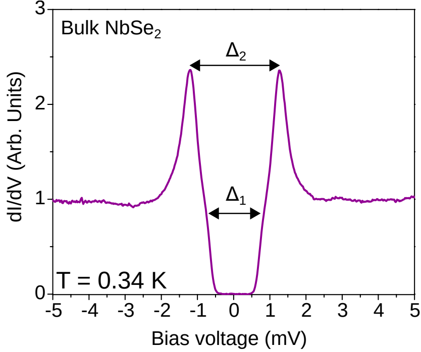
Figure 3.3.3: Low-energy electronic structure of bulk NbSe 2 . Measurement parameters: f = 833 Hz, V_{a.c.} = 30 \mu V.
