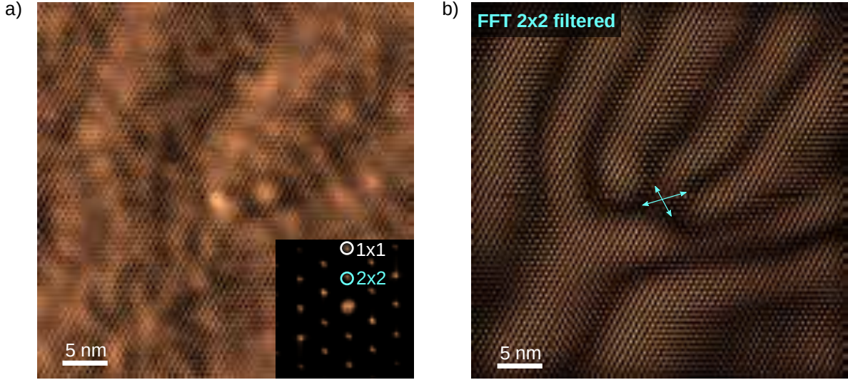
Figure 6.3.1: Atomic structure and CDW modulation in 1T-TiSe 2 /BLG/SiC(0001). a) Atomic resolution STM image ( V_S = -150 mV; I_t = 100 pA; T = 4.2 K). b) Filtered 2 \times 2 CDW components reveals the symmetry of the domain walls.
