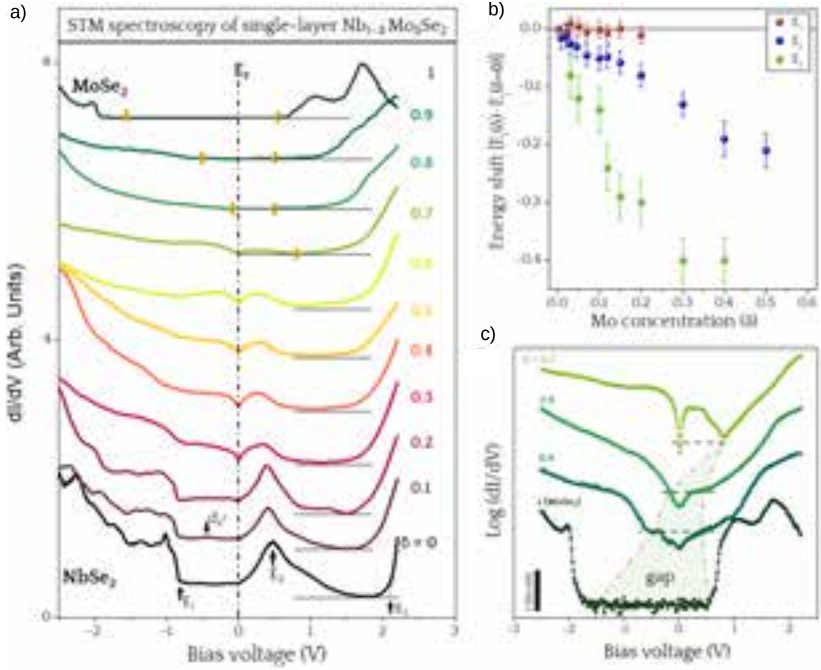
Figure 4.1.8: Electronic structure evolution of the monolayer Nb_{1-\delta}Mo_{\delta}Se_2 alloy. a) Representative wide-bias dI/dV spectra taken on different Nb_{1-\delta}Mo_{\delta}Se_2 monolayers across the full range 0 < \delta < 1 . Each curve represents the averaged electronic structure of alloy areas of 300 - 900 \text{ nm}^2 sampled measuring grids of point dI/dV curves with \sim 2 \text{ curve/nm}^2 . b) Energy shift of the E_{i=1-3} features with respect to their initial energy position in NbSe_2 ( \delta = 0 ) as a function of the Mo concentration ( \delta ). c) Logarithmic plot of the dI/dV spectra relevant for the metal-semiconductor transition ( 0.7 < \delta < 1 ).
