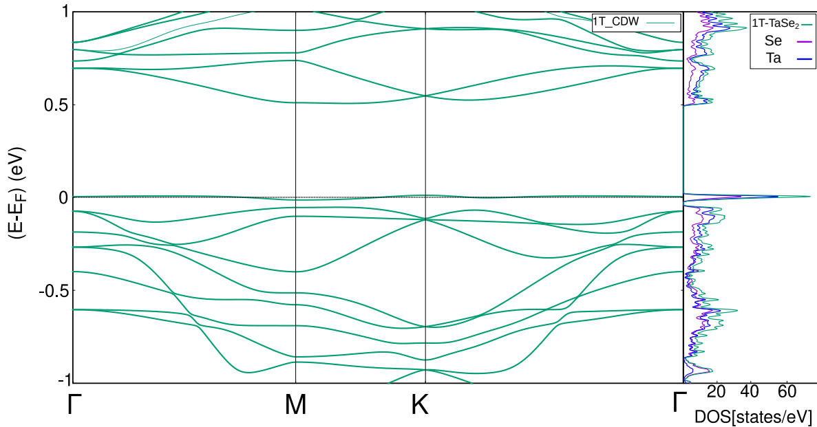
Figure 5.1.6: DFT calculations. (Left) Electronic band structure calculated using the Quantum espresso package within the Perdew-Burke-Ernzerhof approximation. (Right) Calculated DOS.
