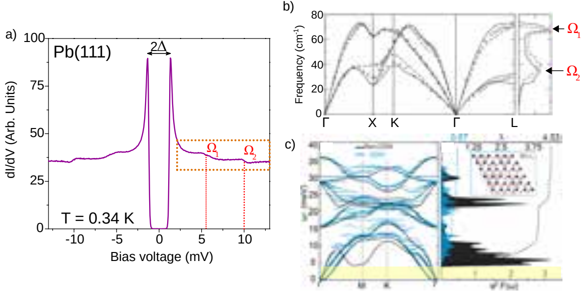
Figure 3.3.9: Virtual phonon features in conventional superconductors. a) STS spectrum acquired around the superconducting gap in Pb(111) at T = 0.34 K ( f = 833 Hz, V_{a.c.} = 50 \mu\text{V} ). The orange box indicates the region where the bosonic modes are seen (shoulder-dip features labelled as \Omega_1 and \Omega_2 ). Both features lie well beyond 2\Delta . b) Phonon dispersion relation of Pb(111) with indicated DOS in the right.[147] c) Phonon dispersion relation of SL-NbSe 2 in the CDW phase combined with the dispersion of the non-CDW phase. The right plot shows the Eliashberg spectra \alpha^2F(\omega) with integrated EPC constants \lambda(\omega) equivalent to the DOS. The yellow region indicates the energy range, where the satellite peaks in the STS measurements of SL-NbSe 2 are observed. As indicated, there are no phonon DOS in this range.[148]
