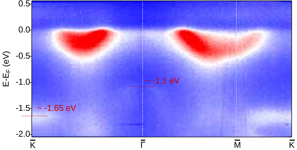
Figure 3.4.7: ARPES band dispersion for SL-NbSe 2 on Au(111) along the high-symmetry \bar{K}-\bar{\Gamma}-\bar{M}-\bar{K} directions. The Nb 4d states cross E_F . In addition, the Se 3p band maxima are faintly visible at \approx -1.1 eV (at \bar{\Gamma} ) and -1.6 eV (near \bar{K} ) below E_F . These band maxima are noted by the red dashed lines, and appear to be consistent with those predicted by theory in Fig. 3.1.2 of section 3.1, specifically the top Se band.
