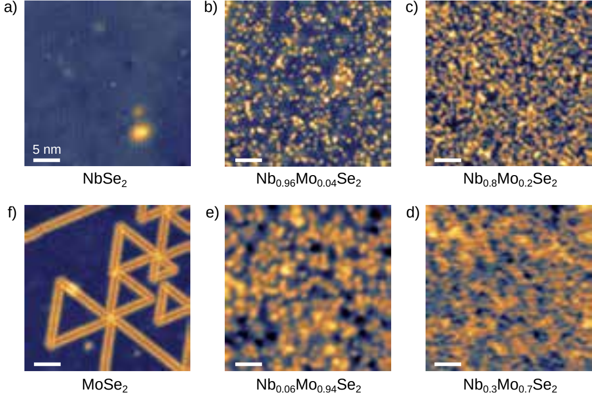
Figure 4.1.5: Atomic-scale morphology evolution of SL-Nb 1-δ Mo δ Se 2 ( 0 < \delta < 1 ). a-f) High resolution STM images of several Nb 1-δ Mo δ Se 2 MLs for different \delta . All the images have the same size for an easier comparison ( 30 \times 30 \text{ nm}^2 ). Imaging parameters: a) V_s = -60 \text{ mV} , I = 580 \text{ pA} , T = 0.34 \text{ K} . b) V_s = -550 \text{ mV} , I = 200 \text{ pA} , T = 0.34 \text{ K} . c) V_s = -500 \text{ mV} , I = 150 \text{ pA} , T = 0.34 \text{ K} . d) V_s = -800 \text{ mV} , I = 10 \text{ pA} , T = 0.34 \text{ K} . e) V_s = -1500 \text{ mV} , I = 20 \text{ pA} , T = 0.34 \text{ K} . f) V_s = -1500 \text{ mV} , I = 50 \text{ pA} , T = 0.34 \text{ K} .
