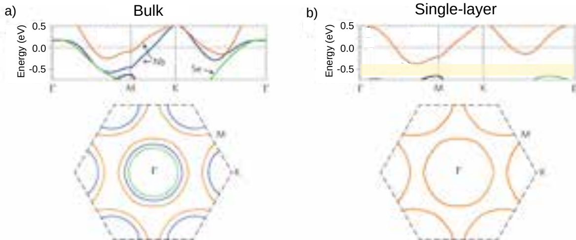
Figure 3.1.3: Comparison of electronic band structure of bulk NbSe 2 and SL-NbSe 2 /BLG/SiC(0001). DFT calculated band structures (top) and Fermi surfaces (bottom) for a) bulk NbSe 2 and b) SL-NbSe 2 /BLG/SiC(0001), respectively. Figure adapted from [6, 119].
