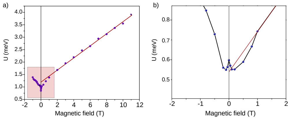
Figure 5.2.6: Gap feature U as a function of the B-field. a) The curve has a linear behaviour in the range of 1 - 11 T. At low B-field (0 - 1 T) the curve shows unexpected non-linearities. b) Another dataset shows a different kind of non-linear behaviour between 0 - 1 T in another location of the unit-cell.
