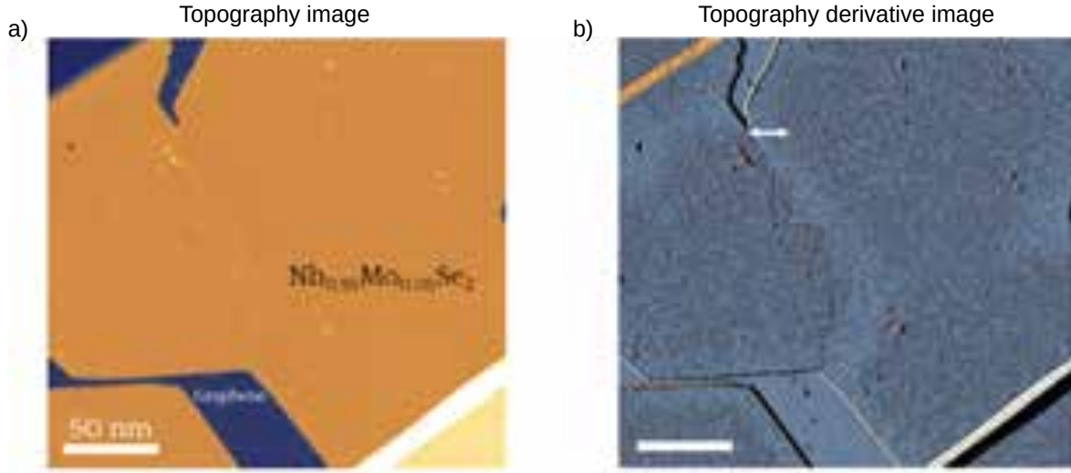
Figure 4.1.6: Homogeneity of the Mo:doped SL-Nb 1- \delta Mo \delta Se 2 alloy. a) Large-scale STM image of the Nb 0.95 Mo 0.05 Se 2 monolayer ( V_s = -0.5 V, I_t = 0.01 nA, T = 4.2 K). b) Topography derivative image of a) to enhance the contrast of the Mo dopant concentration, which is homogenous except for a Mo depletion near the edges of the domains ( \sim 10 nm).
