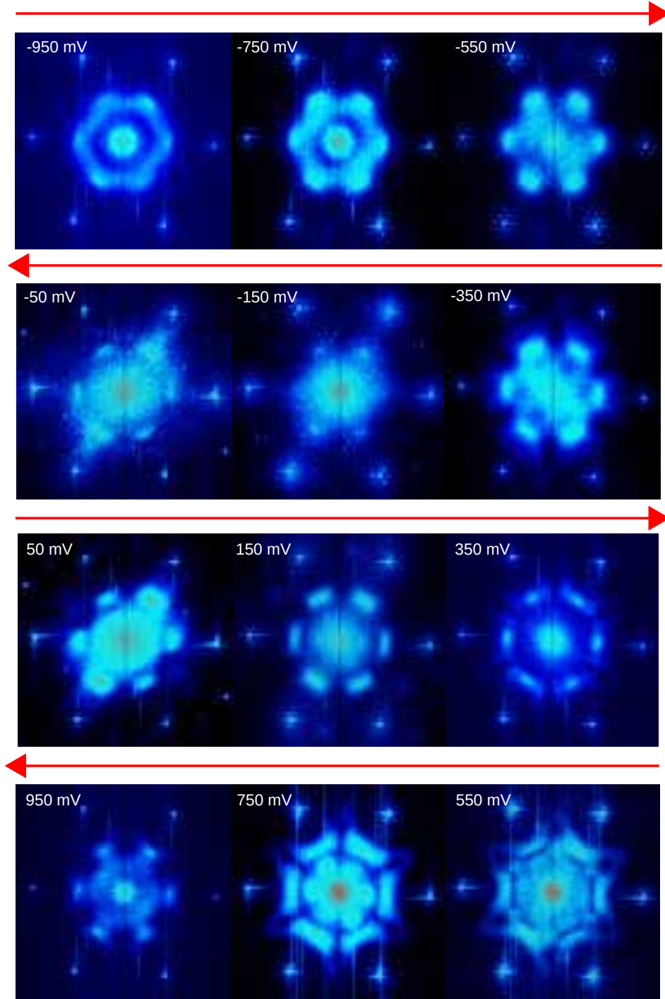
Figure 6.5.1: FFT pattern evolution of SL-TiSe 2 /WSe 2 for different bias voltages. The measured FFT structures are extracted from constant height conductance maps.
