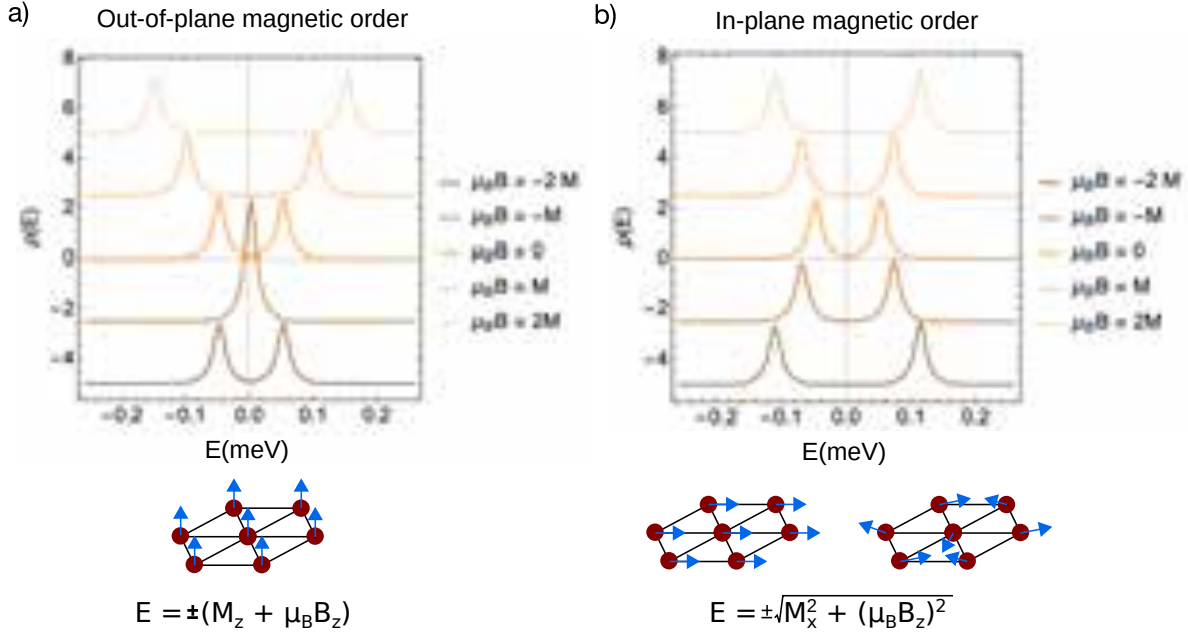
Figure 5.2.8: DOS of magnetically ordered 1T/1H heterostructure. a) If the spins are aligned out-of-plane the gap in the DOS would increase linearly with increasing the field; however, it would decrease for a negative field and eventually close at a critical value of M_z = \mu_B B_z . b) In-plane magnetic order leads to a linear increase of the gap for both polarities, with a non linear behaviour for very small fields of M \ll \mu_B .
