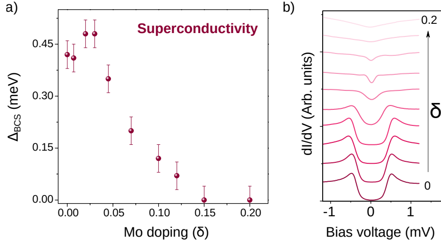
Figure 4.1.11: Superconductivity in the monolayer \text{Nb}_{1-\delta}\text{Mo}_\delta\text{Se}_2 alloy. a) Evolution of the experimental SC gap \Delta with Mo concentration ( \delta ). b) The experimental dI/dV spectra from which the \Delta values are extracted. Each spectrum represents the average over regions of typically \sim 100 \text{ nm}^2 .
