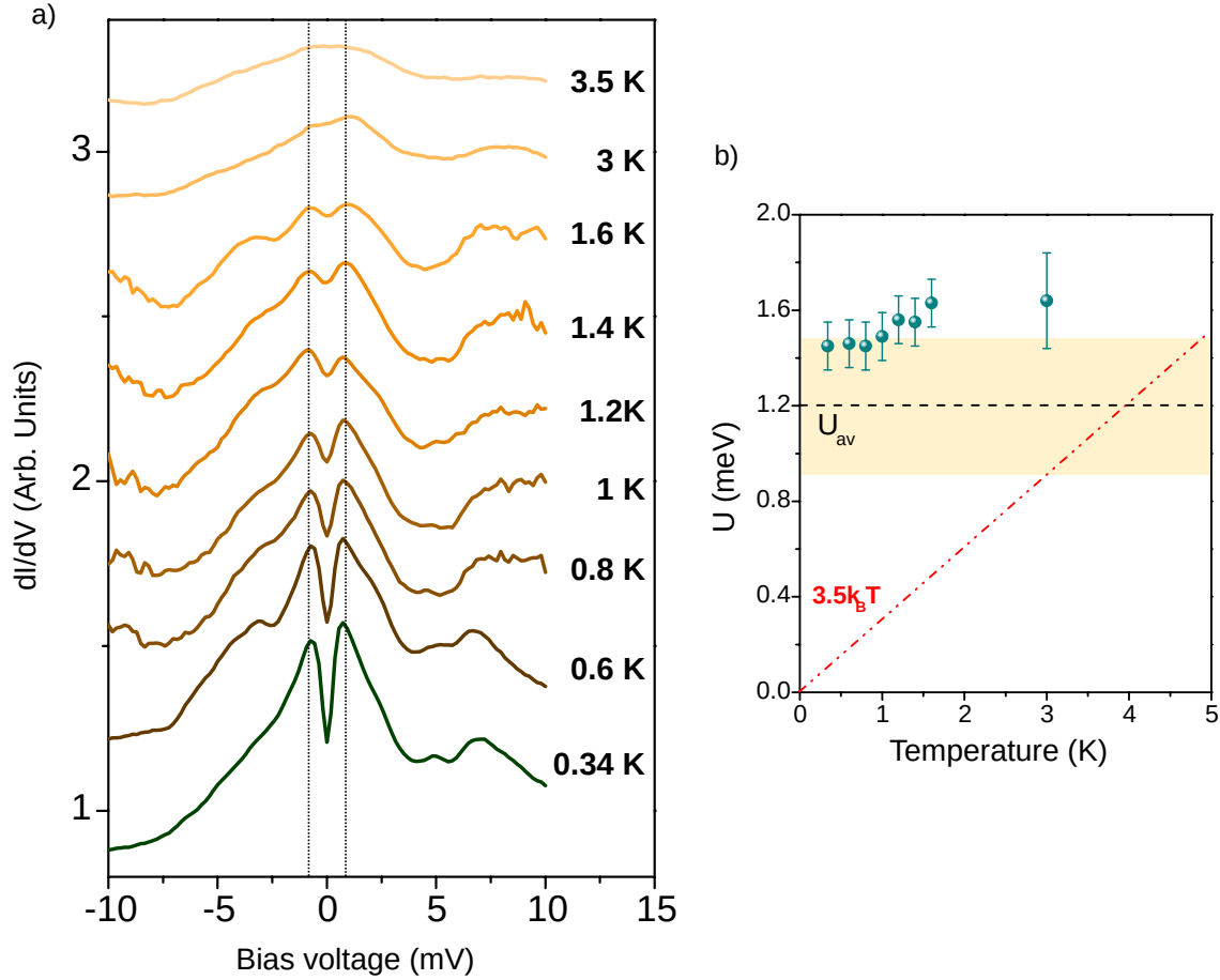
Figure 5.2.4: Temperature dependence of low lying electronic structure of 1T/1H-TaSe 2 . a) Evolution of the dI/dV curves as a function of temperature ( f = 833 Hz, V_{a.c.} = 100 \mu V ). b) The peak separation U for different temperatures.
