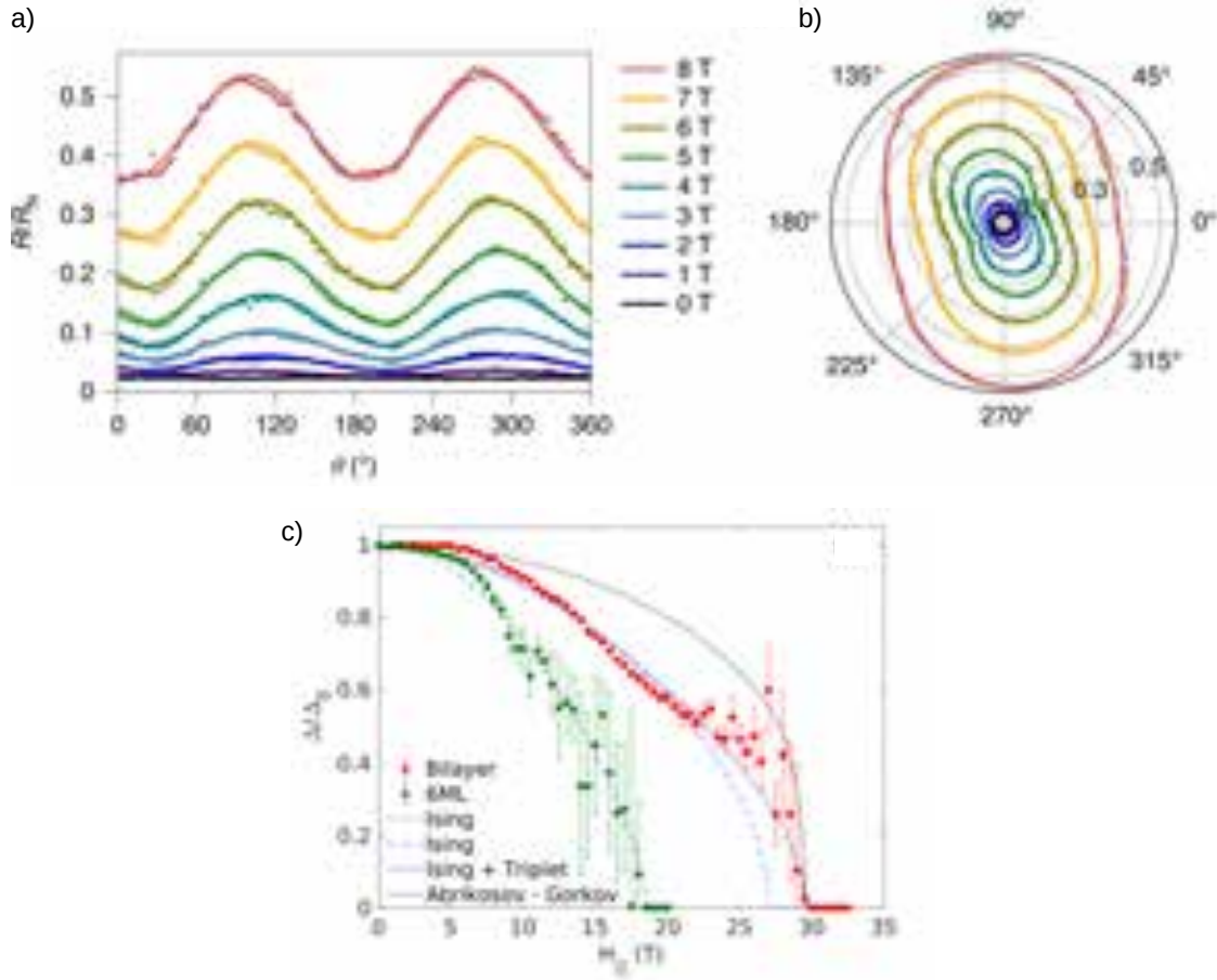
Figure 3.3.1: Closeness of superconducting pairing channels in few layer NbSe 2 . a) Field dependence ( T = 4.2 K) of the magnetoresistance.[123] b) Radial plot of the data in a).[123] c) Normalized superconducting energy gap as a function of the in-plane magnetic field.[125]
