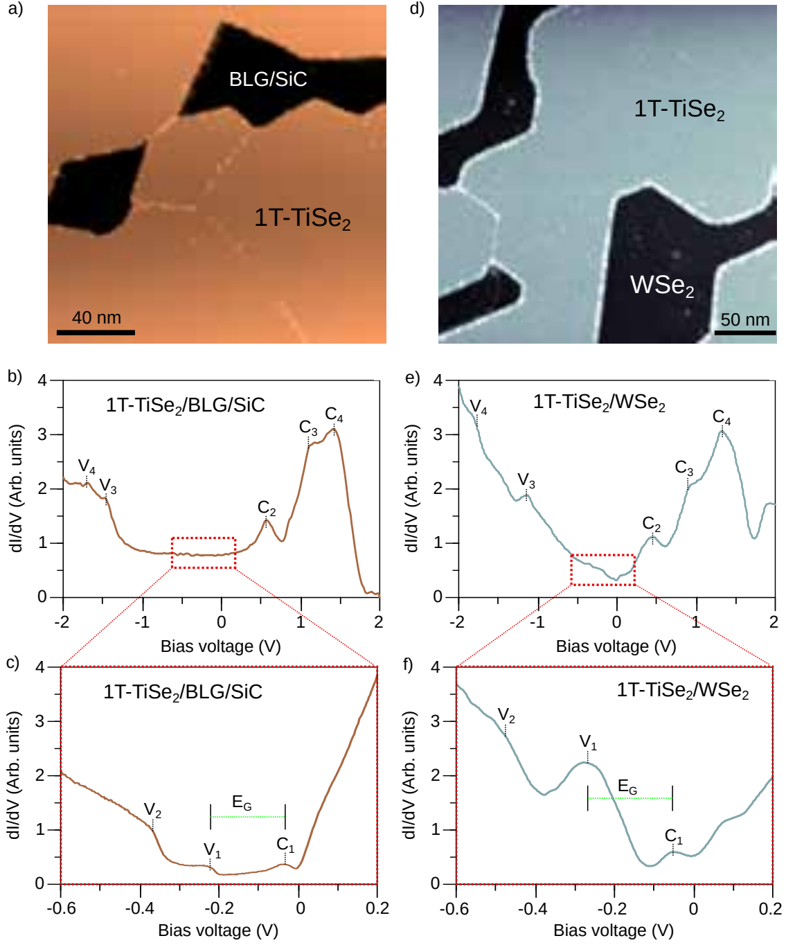
Figure 6.2.1: Topographic (STM) and electronic characterization (STS) of 1T-TiSe 2 . a) Topography ( V_S = +1 V; I_t = 20 pA; T = 4.2 K), b) large scale and c) small scale dI/dV curve of SL-TiSe 2 grown on BLG/SiC. d) Topography ( V_S = +2.8 V; I_t = 8 pA; T = 4.2 K), e) large scale and f) small scale dI/dV curve of SL-TiSe 2 grown on WSe 2 . Measurement parameters: (b,e): f = 833 Hz, V_{a.c.} = 5 mV; (c,f): f = 833 Hz, V_{a.c.} = 0.15 mV.
