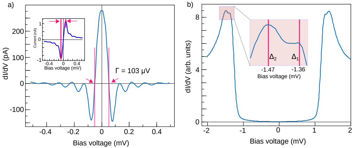
Figure 2.2.7: STS energy resolution measured on Pb(111). a) The width of the Josephson tunneling peak measured with a superconducting tip (Pb) at 0.34 K. The inset shows the I(V) characteristics. b) The dI/dV low lying electronic structure with the two identified superconducting gaps.
