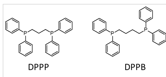
Figure 24. Structure of the selected diphenylphosphino molecules (cross-linkers) to form the intra-chain bond of the SCNPs.
