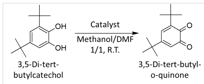
Figure 72. Synthetic scheme of 3,5-di-t-butyl-o-quinone synthesis.
