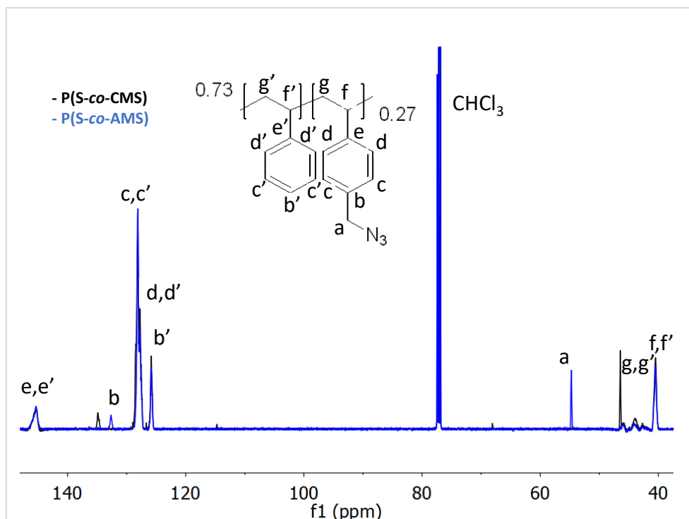
Figure 53. ^{13}\text{C} NMR of P(S-co-CMS) (black) and P(S-co-AMS) (blue).
