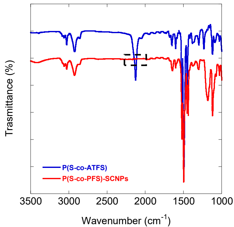
Figure 37. FTIR spectra of P(S-co-ATFS) (blue) and P(S-co-PFS)-SCNPs (red).
