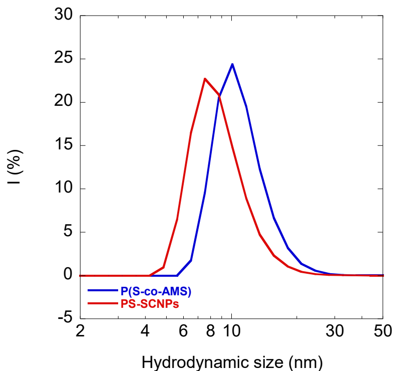
Figure 56. DLS measurement in THF of P(S-co-AMS) (blue) and PS-SCNPs dried (red).
