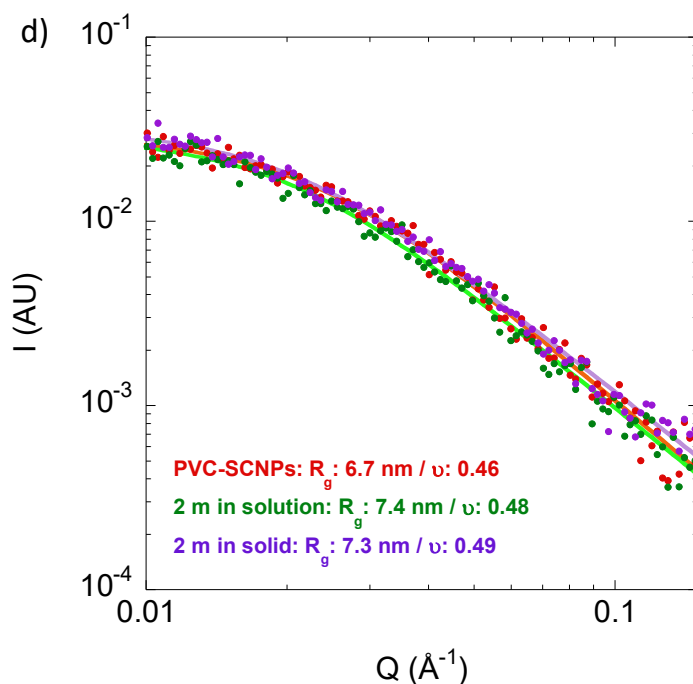
Figure 78. a) GPC chromatogram (LS detector), b) DLS size distribution in THF and SAXS result of the SCNPs after synthesis (c)) and after 2 months of storage (d)). PVC- N_3 in blue, SCNPs after synthesis in red, SCNPs after 2 months of storage in solution in green and SCNPs stored in solid in pink.
