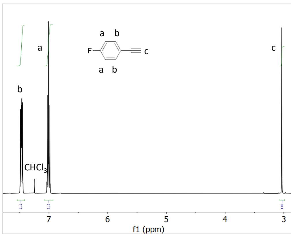
Figure S 15. 1 H NMR spectra of 1-ethynyl-4-fluorobenzene.
