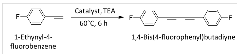
Figure 69. Synthetic scheme of 1,4bis(4-fluorophenyl)butadiyne.
