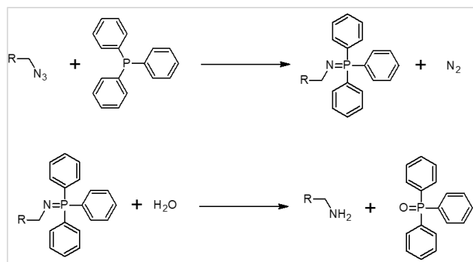
Figure 22. Scheme of the Staudinger reaction’s mechanism.
