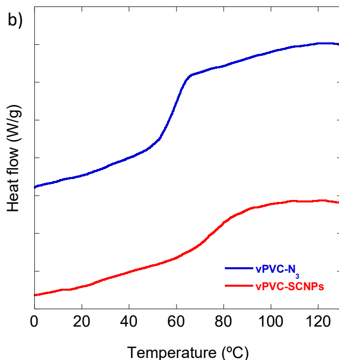
Figure 89. a) TGA and b) DSC traces of vPVC-N 3 in blue and vPVC-SCNPs red. The DSC traces have been downshifted in b) for clarity.
