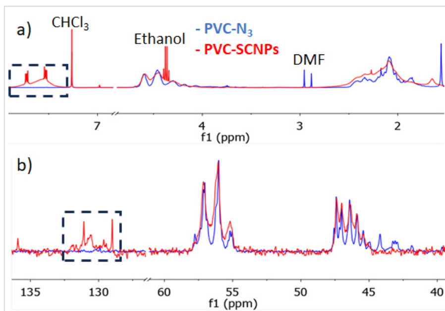
Figure 76. a) ^1\text{H} NMR and b) ^{13}\text{C} NMR of PVC- \text{N}_3 (blue) and PVC-SCNP (red). In the black box are marked the new bands associated to cross linker.
