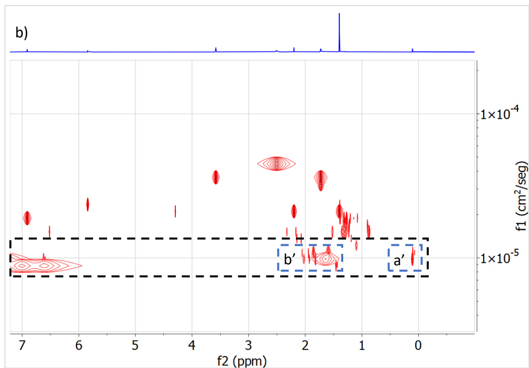
Figure 44. a) ^1\text{H} NMR spectra of TMS (purple) and P(S-co-NTFS) showing the region in which protons from -\text{CH}_3 groups bonded to the silicon atom appear. b) DOSY NMR experiment confirming that the -\text{CH}_3 groups (denoted as a') having the same diffusion coefficient as main chain -\text{CH}_2- and -\text{CH}- protons (denoted as b)- belong to the polymer structure of P(S-co-NTFS).
