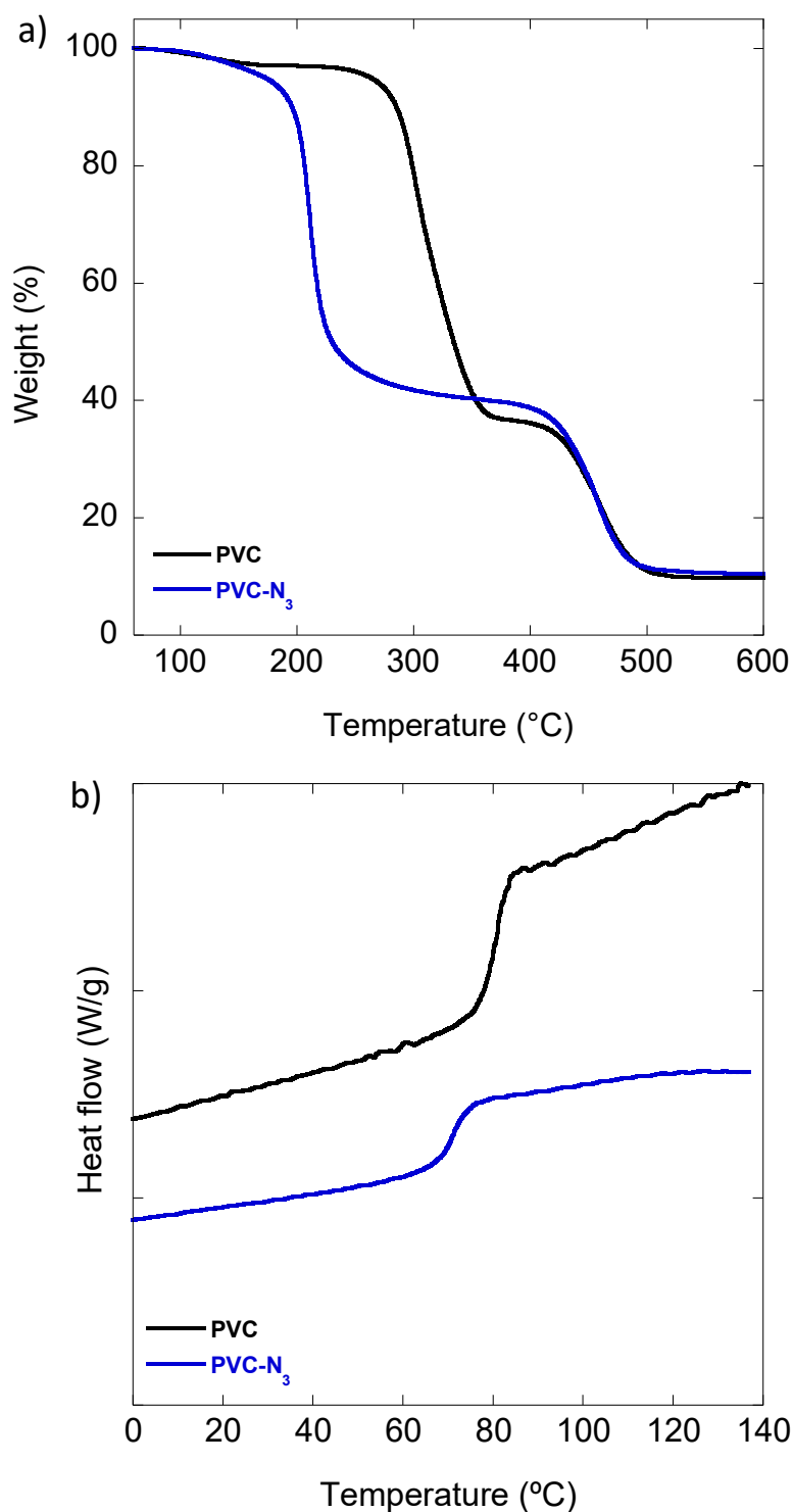
Figure 75. a) TGA and b) DSC traces of PVC (black) and PVC-N 3 (blue).
