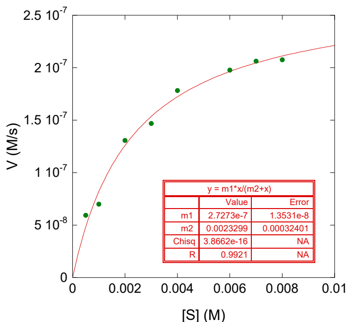
Figure 98. Michaelis-Menten study for reaction with vPVC-SCNPs/Cu(II) as catalyst. Reactions were repeated with different precursor concentrations for the same catalyst concentration.
