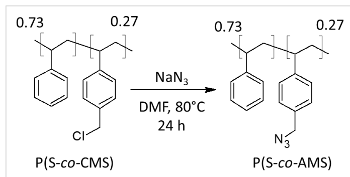
Figure 48. Synthetic scheme of Poly(S-co-AMS).
