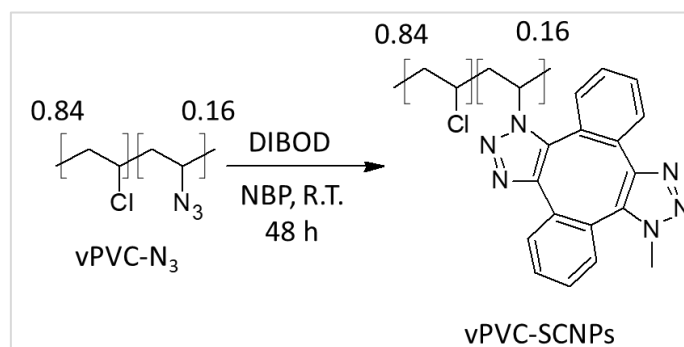
Figure 66. Synthetic scheme of vPVC-SCNPs.
