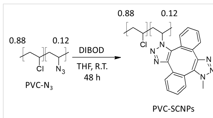
Figure 64. Synthetic scheme of PVC-SCNPs.
