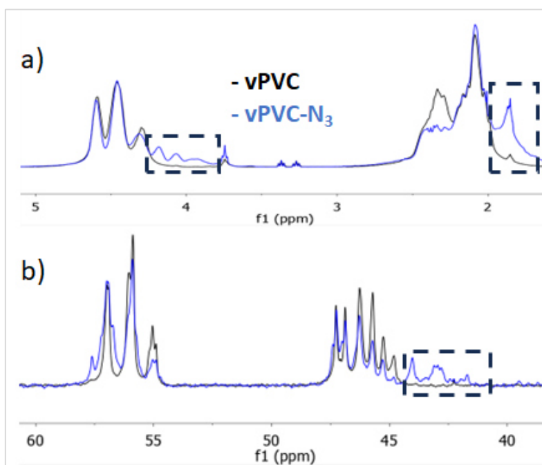
Figure 83. a) 1 H NMR and b) 13 C NMR spectra of vPVC (black) and vPVC-N 3 (blue). In the black boxes are marked the new bands associated to vPVC-N 3 .
