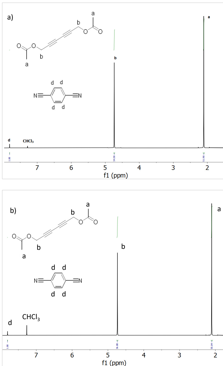
Figure 92. Leaching experiment. ^1\text{H} NMR spectra of the hexa-2,4-diyne-1,6-diyl diacetate synthesized with vPVC-SCNPs/Cu(II) a) for 3 hours and b) for another additional 3 hours after remove the vPVC-SCNPs/Cu(II) catalyst .
