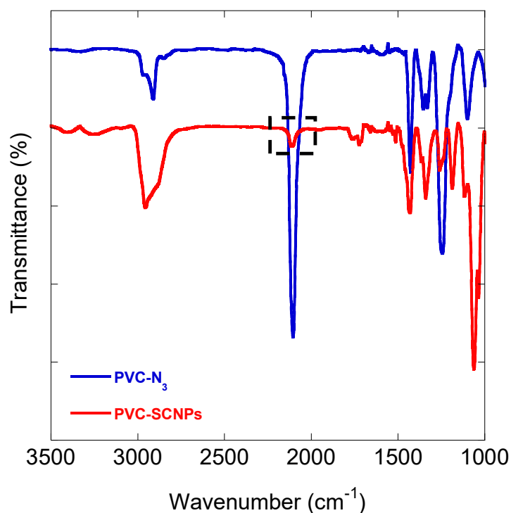
Figure 77. FTIR spectra of PVC- \text{N}_3 (blue) and PVC-SCNP (red). In the black box is marked the peak associated to the azide group.
