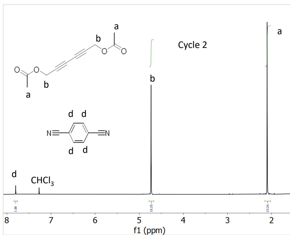
Figure S 10. 1 H NMR spectra of the hexa-2,4-diyne-1,6-diyl diacetate synthesized with vPVC-SCNPs/Cu(II) at the second cycle.
