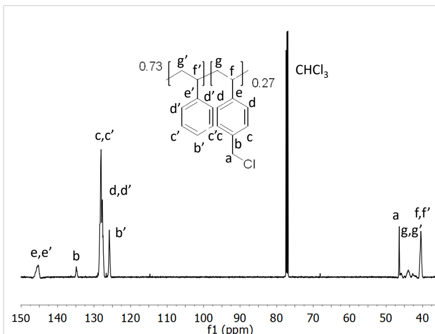
Figure 51. ^{13}\text{C} NMR spectrum of P(S-co-CMS).
