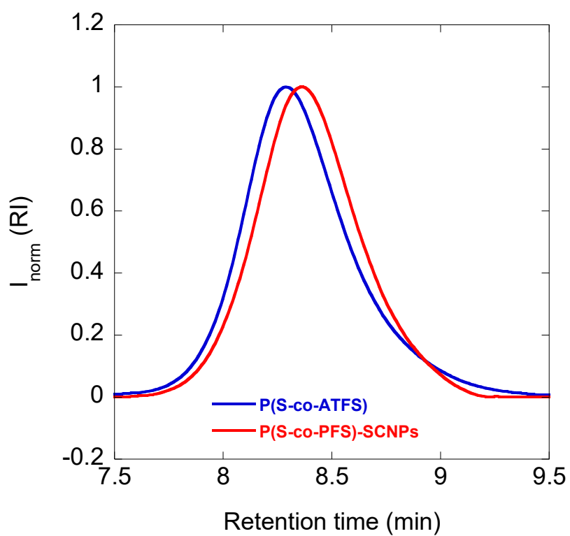
Figure 34. GPC chromatogram (RI detector) of P(S-co-ATFS) (blue) and P(S-co-PFS)-SCNPs (red) (RI signal).
