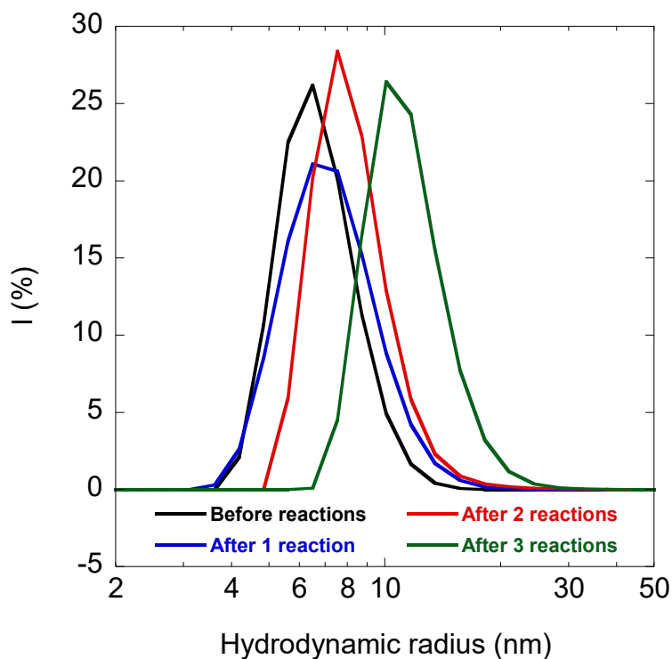
Figure 93. DLS size distribution in THF of vPVC-SCNPs/Cu(II) before the catalysis reactions (black) and after 1 (blue), 2 (red) and 3 (green) reactions.
