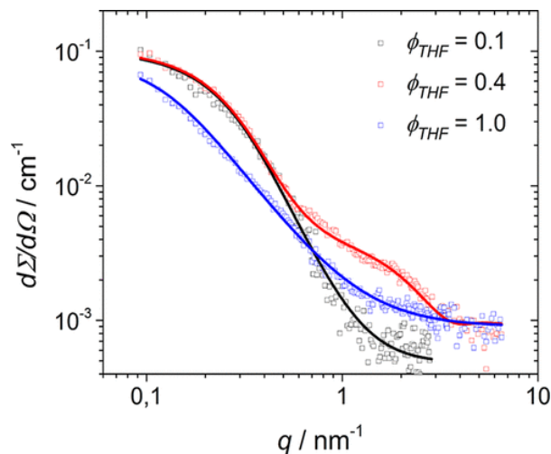
Figure 10. SAXS results in various solvent compositions, showing the compaction differences in function of the solvent [62]. As \phi_{THF} = 0.1 and \phi_{THF} = 0.4 are not good solvent for the sample the result shows a compaction in these cases.
