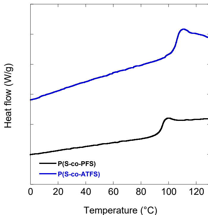
Figure 33. DSC of P(S-co-PFS) (black) and P(S-co-ATFS) (blue).
