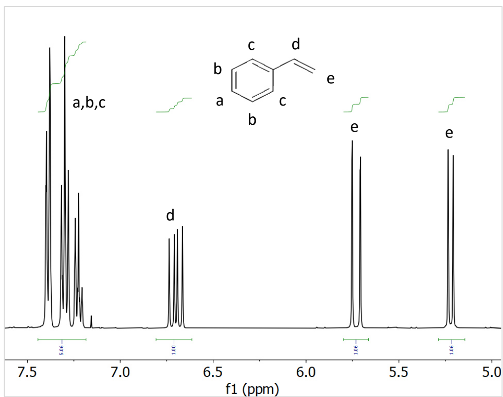
Figure S 17. ^1\text{H} NMR spectra of styrene.
