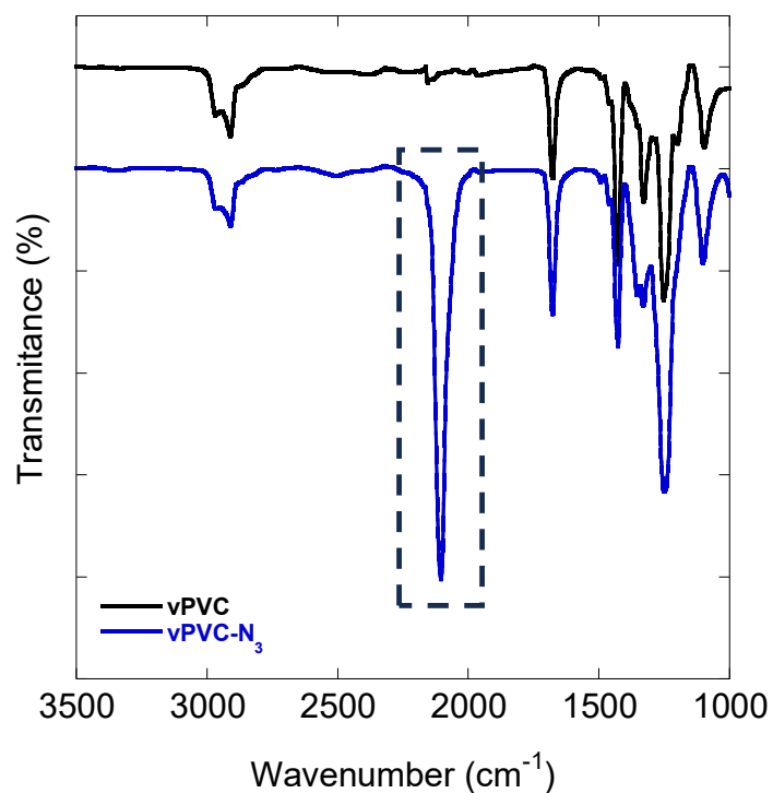
Figure 84. FTIR spectra of vPVC in black and vPVC-N 3 in blue. The new peak related with the azide group is marked with the black box.
