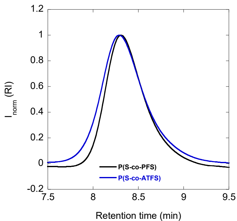
Figure S 2. GPC chromatogram (RI detector) and of P(S-co-PFS) (black) and P(S-co-ATFS) (blue) (RI signal).
