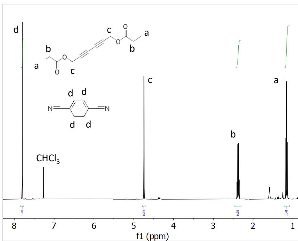
Figure S 14. 1 H NMR spectra of 2,4-hexadiyne-1,6-diol dipropionate synthesized with CuCl 2 (model reaction).
