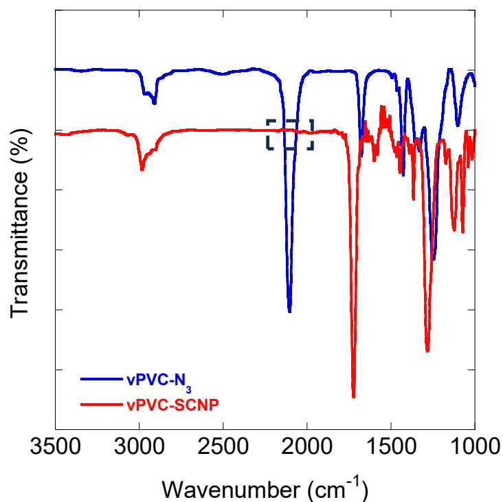
Figure 87. FTIR spectra of vPVC- \text{N}_3 (blue) and vPVC-SCNP (red). In the black box is marked the peak associated to the azide group.
