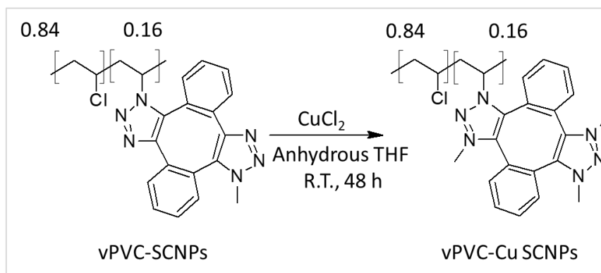
Figure 67. Synthetic scheme of vPVC-Cu SCNPs.
