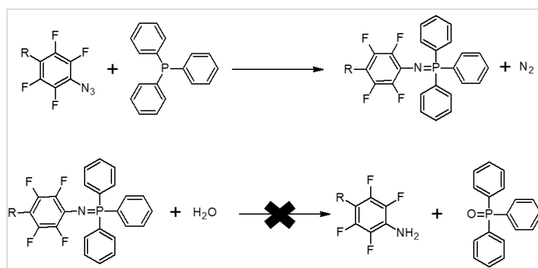
Figure 23. Scheme of the frustrated Staudinger reaction, avoiding the hydrolyzation of the azaylide bond.
