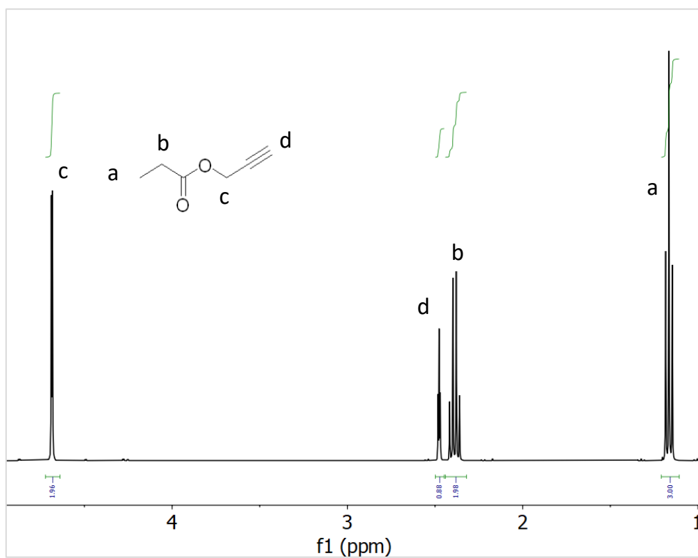
Figure S 13. 1 H NMR spectra of propargyl propionate.
