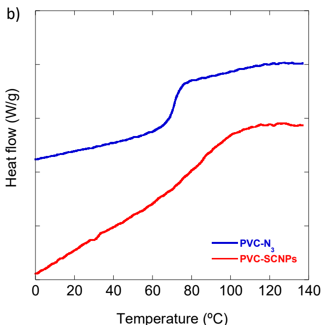
Figure 79. a) TGA and b) DSC traces of PVC-N 3 (blue) and PVC-SCNPs (Red). The DSC traces have been downshifted for clarity.
