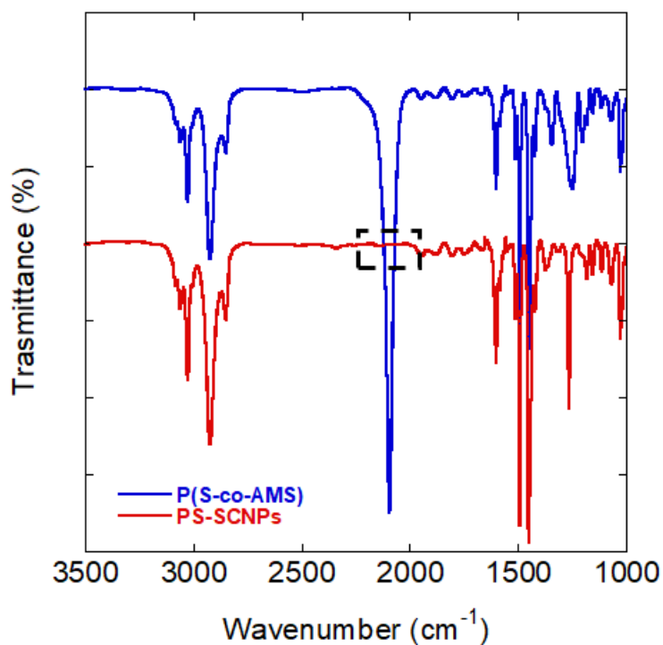
Figure 59. FTIR spectra of P(S-co-AMS) (blue) and PS-SCNPs (red). The new peak associated with the azide group is marked with the black box.
