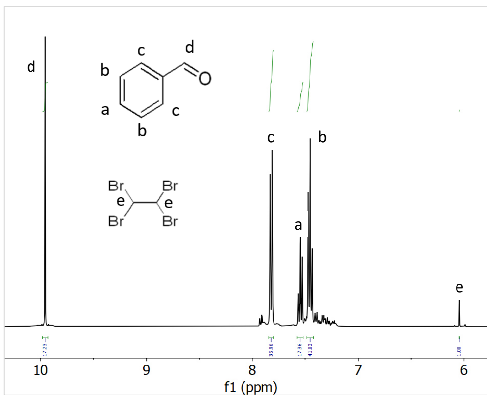
Figure S 18. ^1\text{H} NMR spectra of benzaldehyde synthesized with \text{CuCl}_2 (model reaction).
