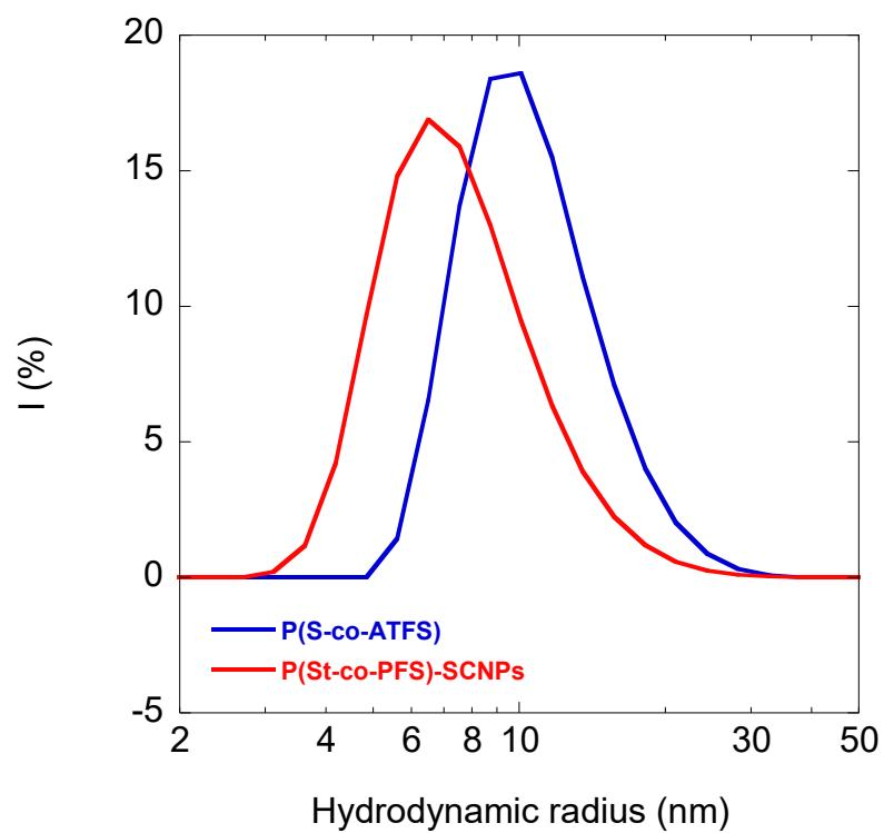
Figure 35. DLS size distribution in THF of P(S-co-ATFS) (blue) and P(S-co-PFS)-SCNPs (red).
