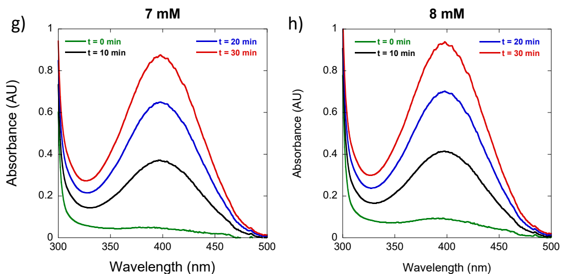
Figure S 19. Kinetics experiments to assess for Michaelis–Menten behavior of vPVC-SCNPs/Cu(II) in the oxidation of DTBC to DTBQ with substrate concentrations ranging from 0.5 mM to 8 mM and identical concentration of vPVC-SCNPs/Cu(II) catalyst ( [\text{Cu(II)}] = 4.8 \mu\text{M} ).
