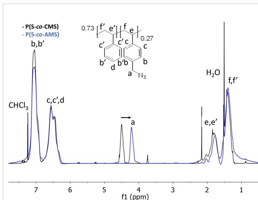
Figure 52. ^1\text{H} NMR spectra of P(S-co-CMS) (black) and P(S-co-AMS) (blue).
