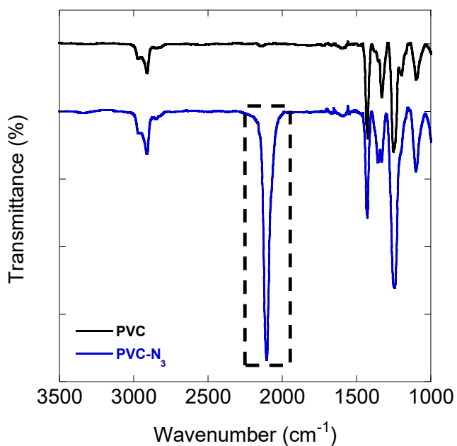
Figure 74. FTIR spectra of PVC in black and PVC- \text{N}_3 in blue. The new peak associated with the azide group is marked with the black box.
