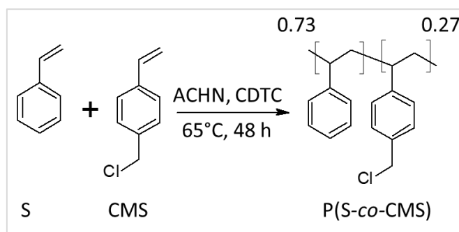
Figure 47. Synthetic scheme of P(S-co-CMS).
