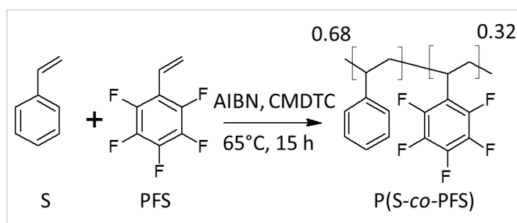
Figure 25. Synthetic scheme of P(S-co-PFS).
