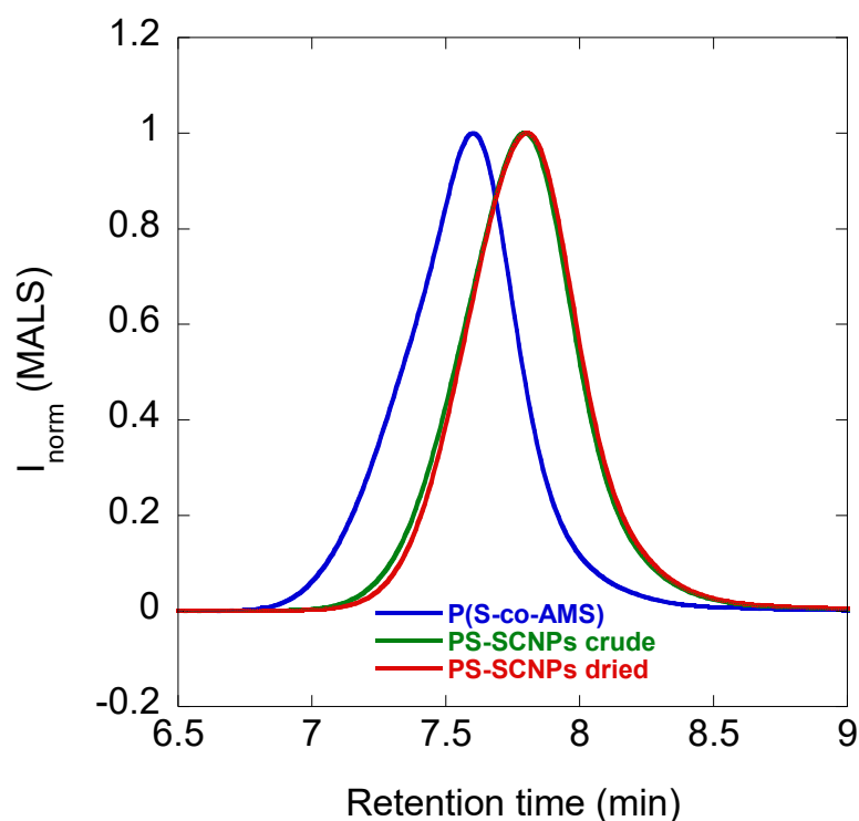
Figure 55. GPC chromatograph of P(S-co-AMS) (blue), PS-SCNPs crude (green) and PS-SCNPs dried (red) (LS detector).
