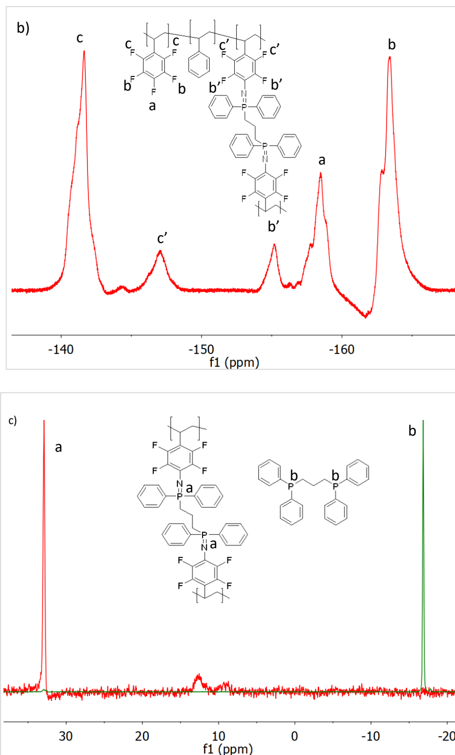
Figure 38. NMR spectra of P(S-co-PFS)-SCNPs (red) and DPPP (green). a) ^1\text{H} NMR, showing the new peaks f and g related with the cross-linker. b) ^{19}\text{F} NMR showing the new peaks b' and c'. c) ^{31}\text{P} NMR, showing the shift of the peak of the cross-linker before and after the reaction.
