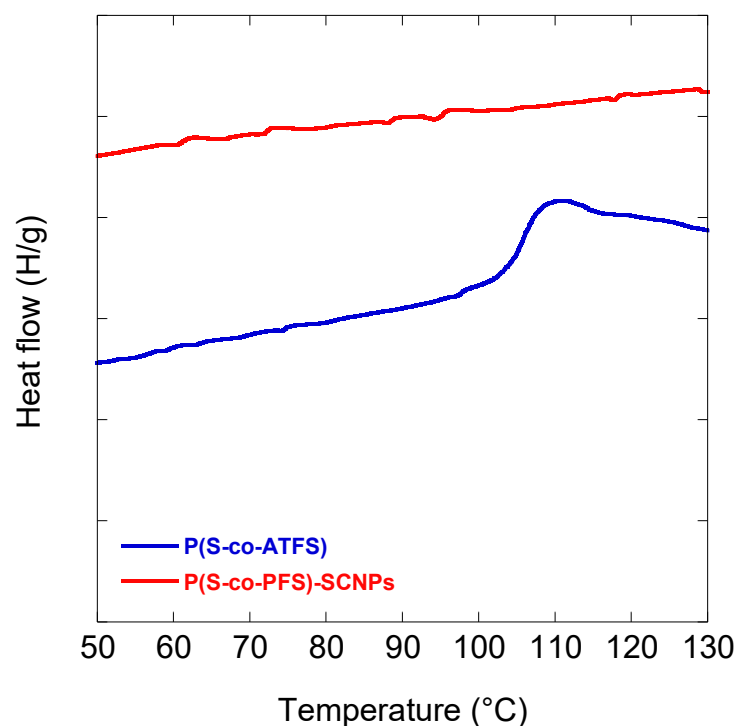
Figure 40. DSC results of P(S-co-ATFS) (blue) and P(S-co-PFS)-SCNPs (red).
