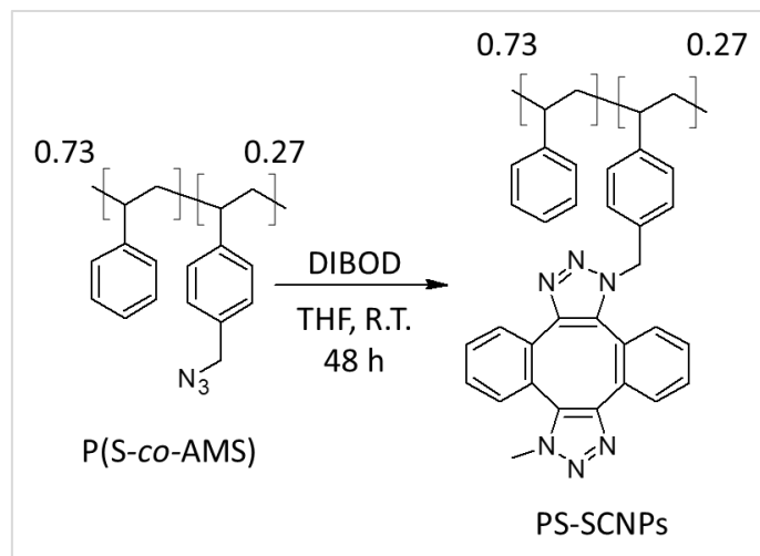
Figure 49. Synthetic scheme of PS-SCNPs.
