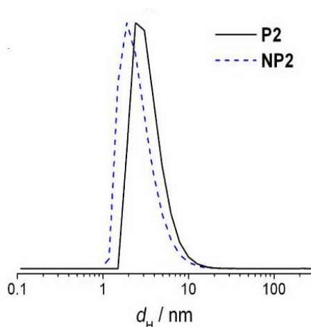
Figure 9. DLS result showing the size reduction of the SCNPs (NP2) from the polymer precursor (P2) [57].
