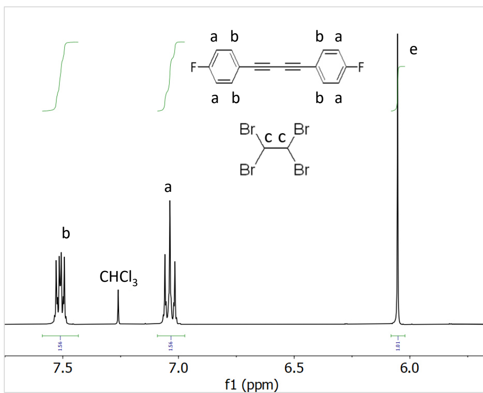
Figure S 16. 1 H NMR spectra of 1,4-bis(4-fluorophenyl)butadiyne synthesized with CuCl 2 (model reaction).
