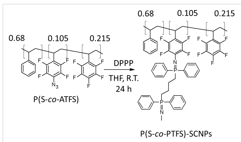
Figure 27. Synthetic scheme of P(S-co-PFS)-SCNPs.
