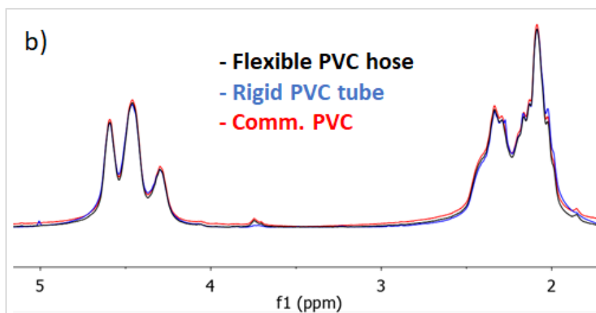
Figure 82. a) GPC chromatograph (RI detector) and b) ^1\text{H} NMR spectra of the valorized and commercial PVC. PVC from flexible hose in black, from rigid tube in blue and commercial in red.
