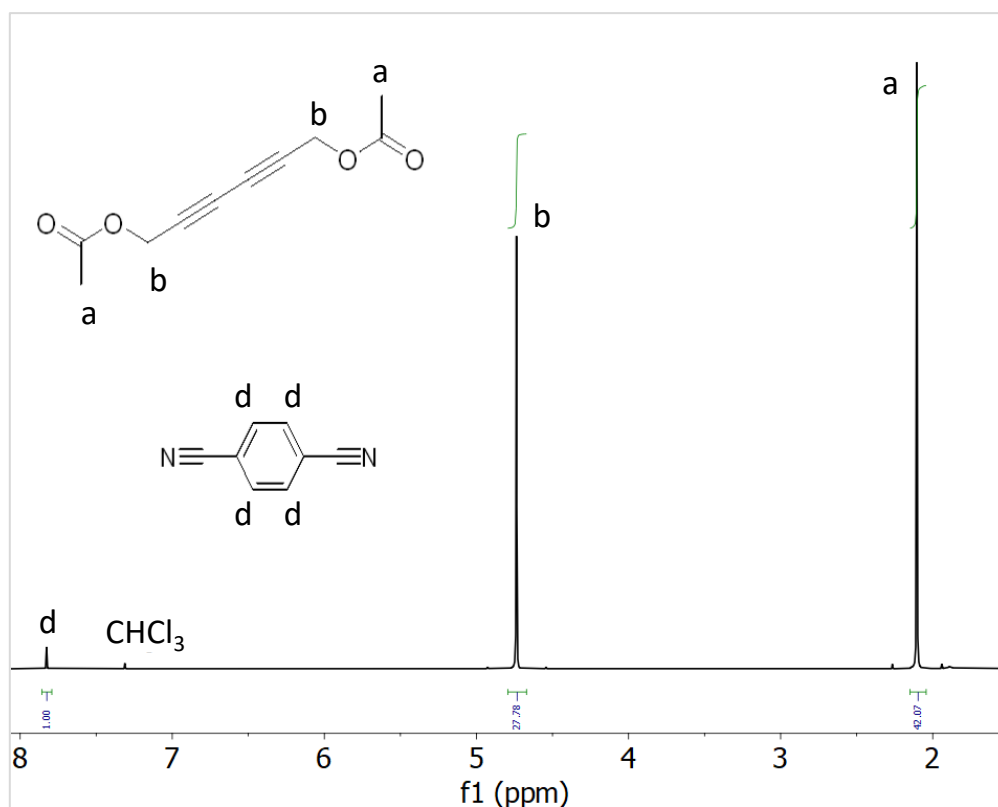
Figure S 9. 1 H NMR spectra of the hexa-2,4-diyne-1,6-diyl diacetate synthesized, as a model reaction, with CuCl 2 .
