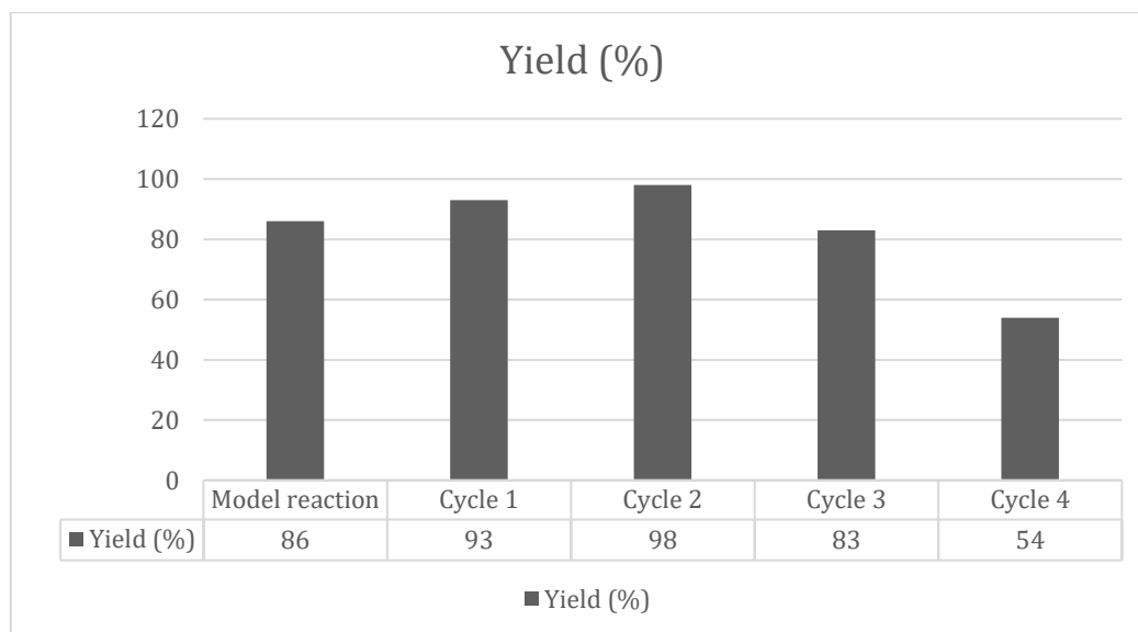
Figure 91. Graph of the yields of the hexa-2,4-diyne-1,6-diyl diacetate synthesis reactions showing the comparison between model reaction and each cycle reaction with PVC-Cu SCNPs.
