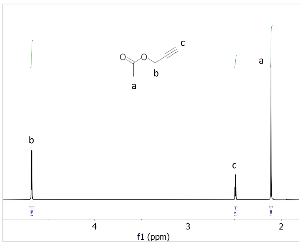
Figure S 8. 1 H NMR spectra of propargyl acetate, the reagent of the reaction.
