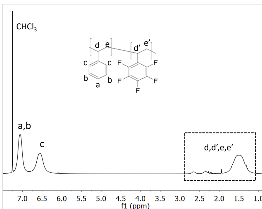
Figure 28. 1 H NMR spectra of P(S-co-PFS).
