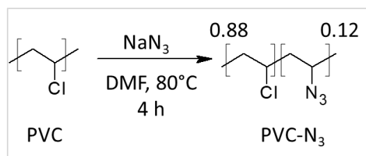
Figure 63. Synthetic scheme of PVC-N 3 .
