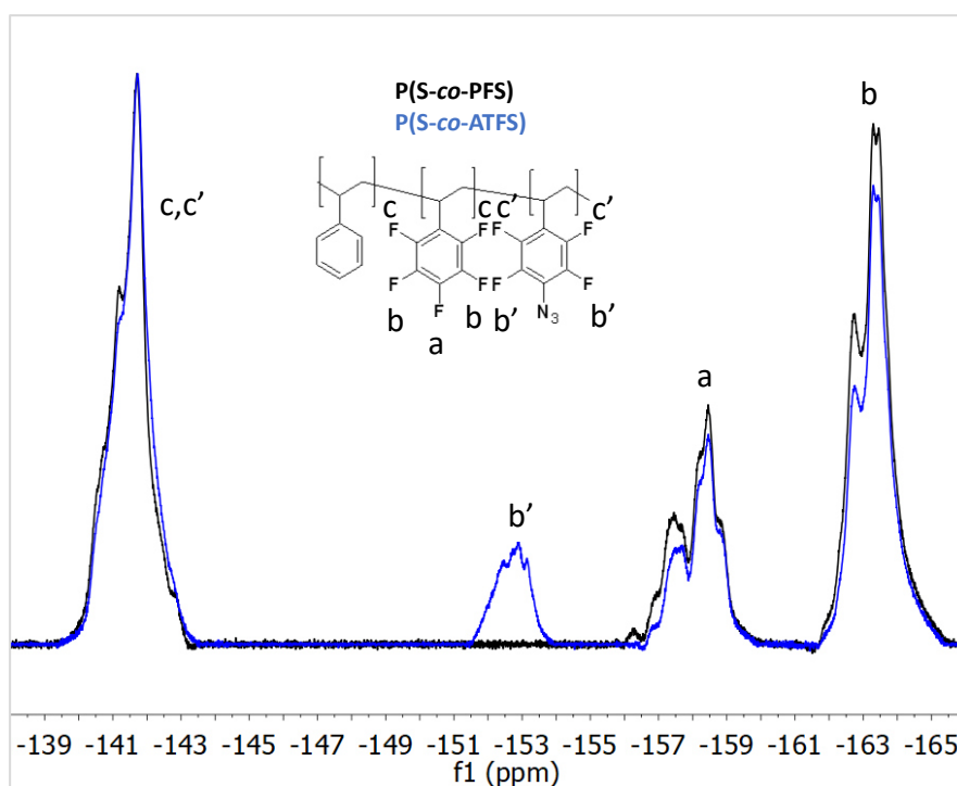
Figure 31. ^{19}\text{F} NMR spectra of P(S-co-PFS) (black) and P(S-co-ATFS) (blue).
