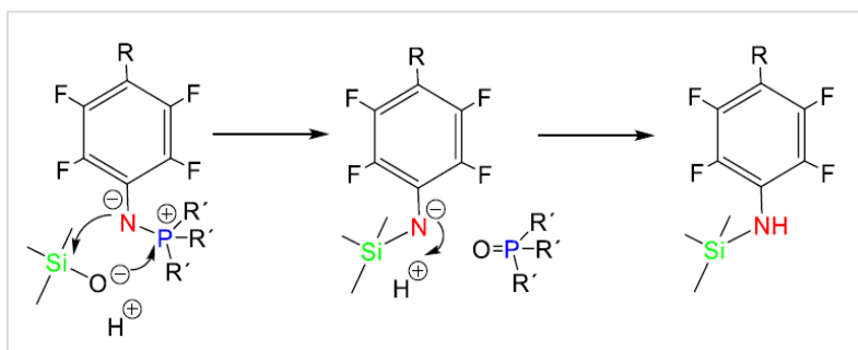
Figure 45. Scheme of the tentative mechanism of the TMS triggered stable azaylide rupture reaction.
