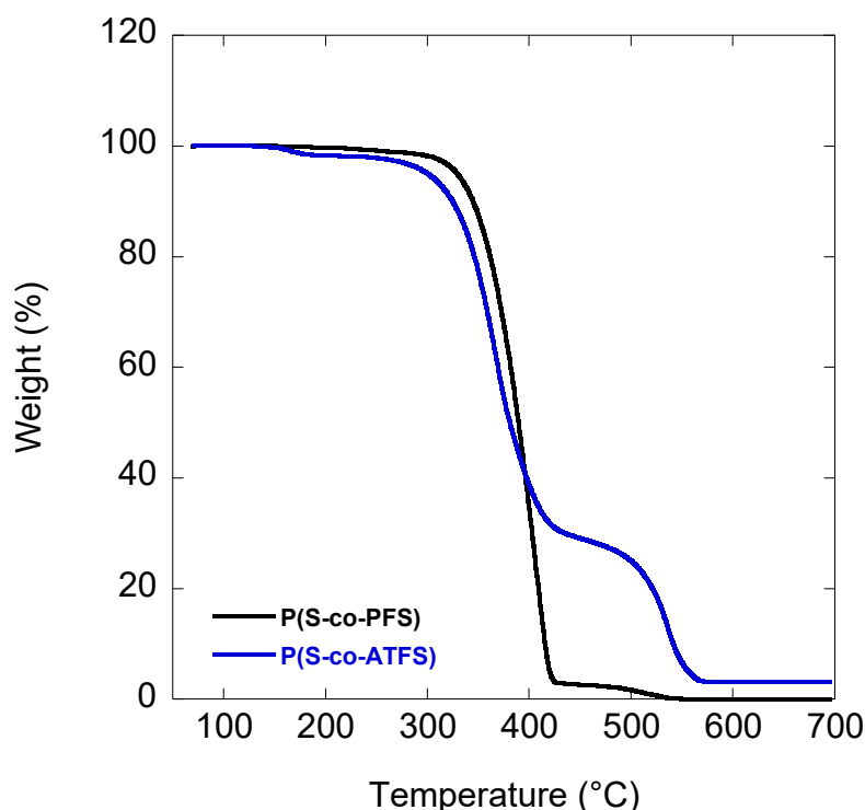
Figure 32. TGA of P(S-co-PFS) (black) and P(S-co-ATFS) (blue).
