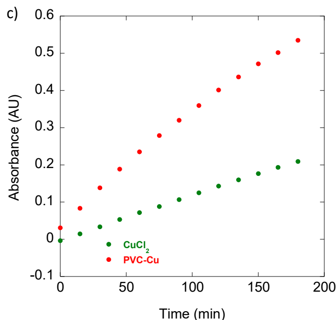
Figure 97. a) UV-Vis spectra and of the 3,5-di-butyl-o-quinone synthesis with vPVC-SCNPs/Cu(II) as catalyst (model reaction), b) UV-Vis spectra and of the 3,5-di-butyl-o-quinone synthesis with CuCl 2 as catalyst and c) comparison of the absorbance at 400 nm synthesis with CuCl 2 (green) and vPVC-SCNPs/Cu(II) (red) as catalyst.
