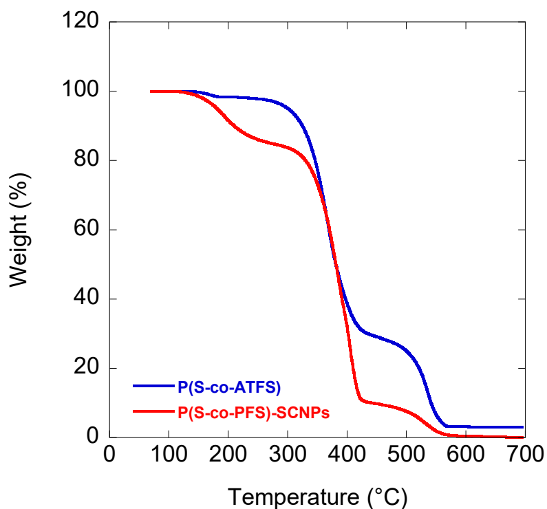
Figure 39. TGA results of P(S-co-ATFS) (blue) and P(S-co-PFS)-SCNPs (red).
