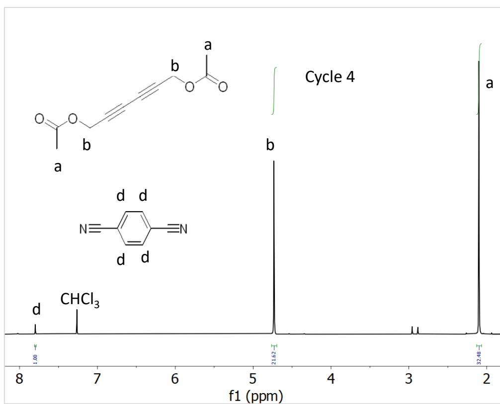
Figure S 12. ^1\text{H} NMR spectra of the hexa-2,4-diyne-1,6-diyl diacetate synthesized with vPVC-SCNPs/Cu(II) at the fourth cycle.
