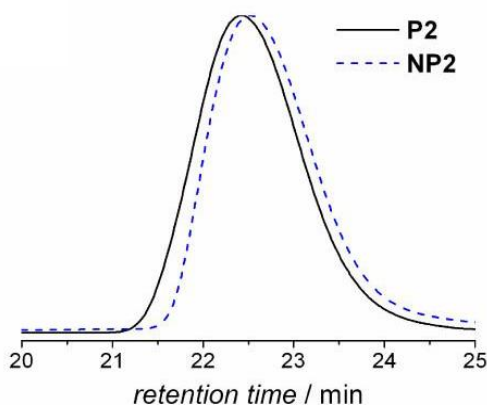
Figure 8. GPC chromatogram showing the size reduction of the SCNPs (NP2) from the polymer precursor (P2) [57].
