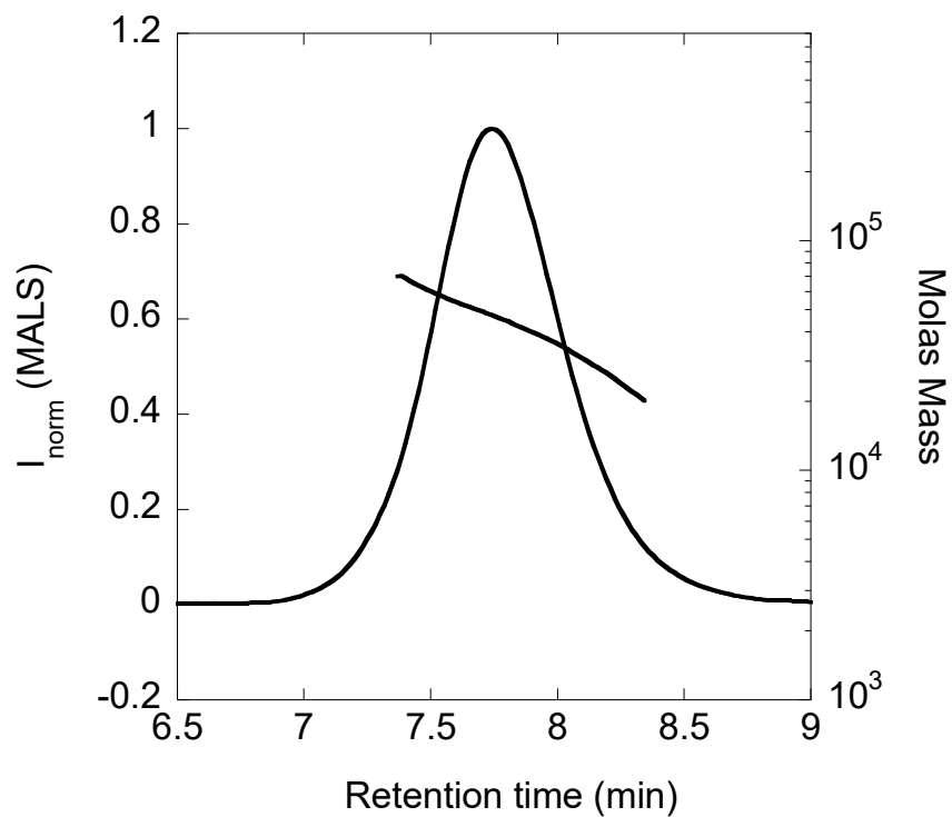
Figure S 1. GPC chromatogram of P(S-co-PFS) (LS signal).
