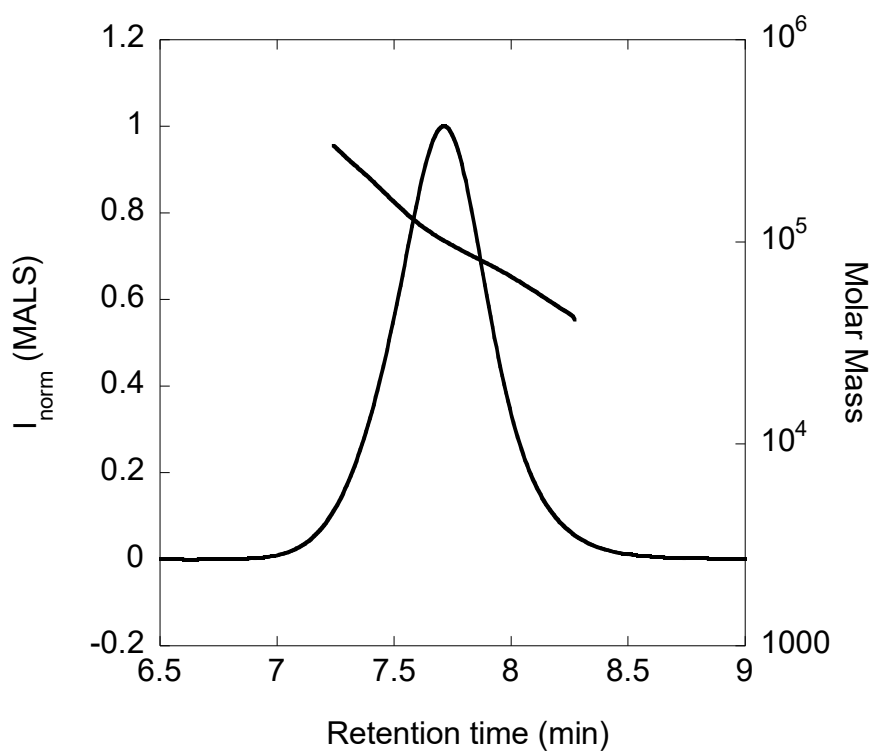
Figure S 5. GPC chromatograph of P(S-co-CMS) (LS detector).
