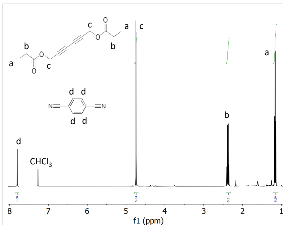
Figure 94. ^1\text{H} NMR spectra of 2,4-hexadiyne-1,6-diol dipropionate synthesized with vPVC-SCNPs/Cu(II).
