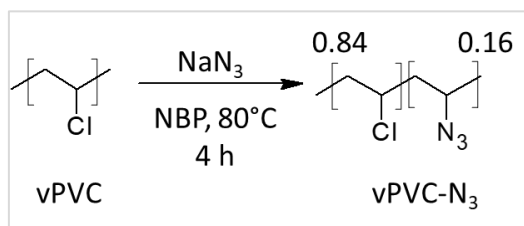
Figure 65. Synthetic scheme of vPVC-N 3 .
