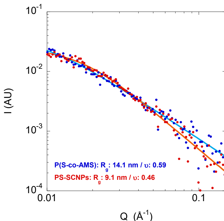
Figure 57. Experimental data (points) and fitting (line) of the SAXS characterization of P(S-co-AMS) (blue) and PS-SCNPs dried (red). Values of R_g and v were obtained through fits of the experimental data to a generalized Gaussian coil function.
