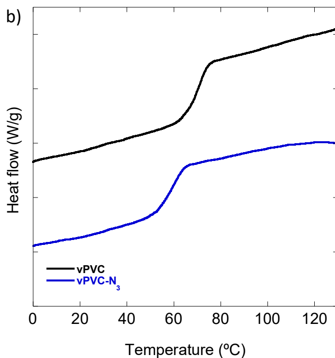
Figure 85. a) TGA and b) DSC traces of vPVC (black) and vPVC-N 3 (blue). The DSC traces have been downshifted for clarity.
