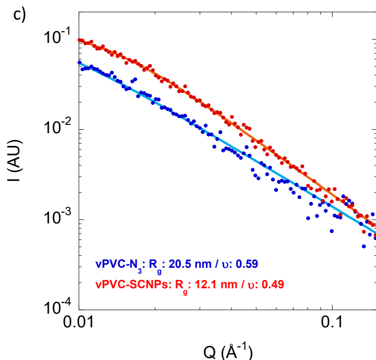
Figure 88. a) GPC chromatogram (RI detector), b) DLS size distribution in THF, c) SAXS result of vPVC- N_3 in blue and vPVC-SCNPs red.
