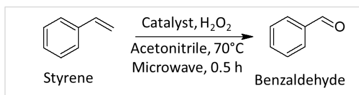
Figure 71. Synthetic scheme of benzaldehyde.
