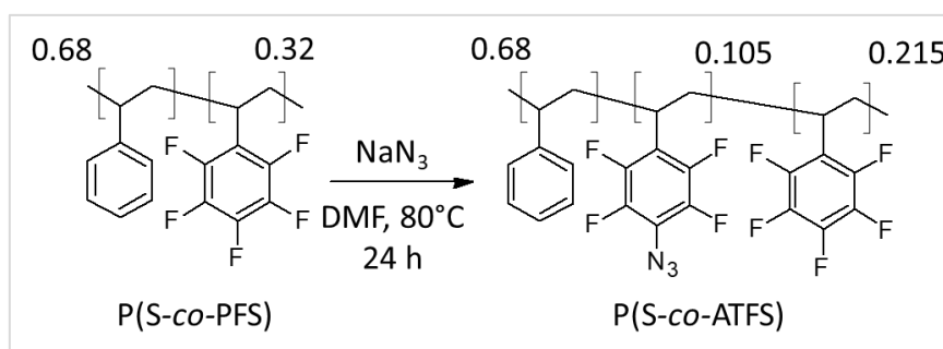
Figure 26. Synthetic scheme of P(S-co-ATFS).
