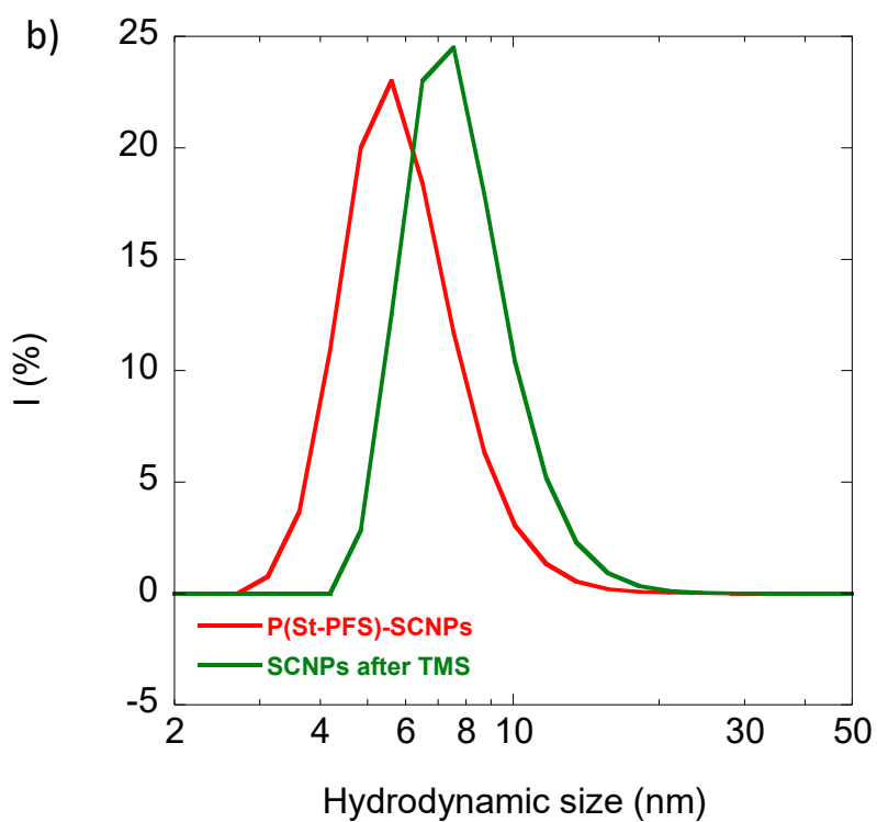
Figure 42. a) GPC chromatogram (RI detector) and b) DLS size distribution in THF of P(S-co-ATFS) (blue), P(S-co-PFS)-SCNPs (red) and P(S-co-PFS)-SCNPs after been exposed to TMS for 3 days.
