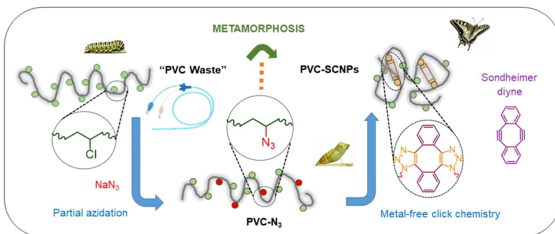
Figure 62. Metamorphosis of “PVC waste” to PVC Single-Chain Nanoparticles (PVC-SCNPs) in two steps: i) partial azidation of PVC to PVC-N 3 ; and ii) intra-chain metal-free click chemistry at r.t. involving individual PVC-N 3 chains and the Sondheimer diyne (5,6,11,12-tetradehydrodibenzo[a,e]cyclooctene) to give PVC-SCNPs.
