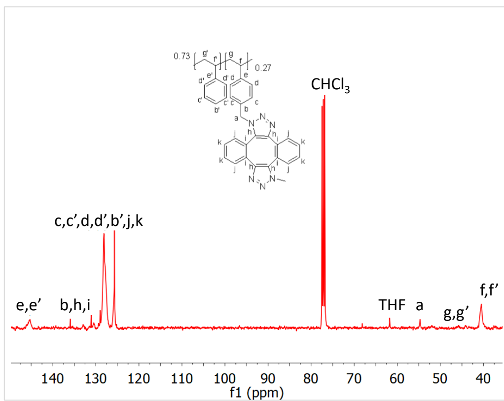
Figure S 6. ^{13}\text{C} NMR of PS-SCNPs. The new peaks h, i, j and k correspond to the cross-linker.
