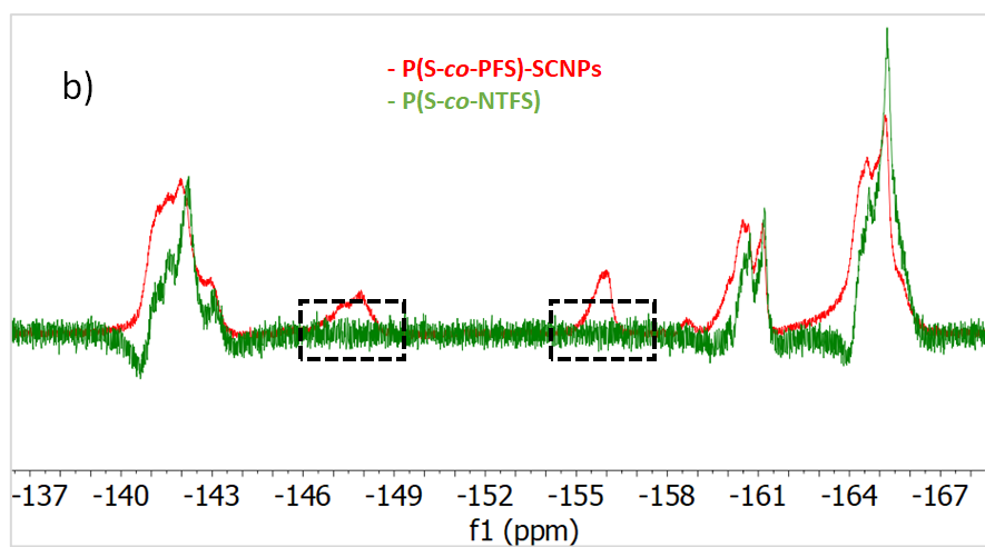
Figure 43. a) FTIR spectra and b) ^{19}\text{F} spectra of P(S-co-PFS)-SCNPs (red) and P(S-co-NTFS) (green).
