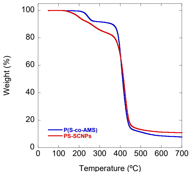
Figure 60. TGA result of P(S-co-AMS) (blue) and PS-SCNPs (red).
