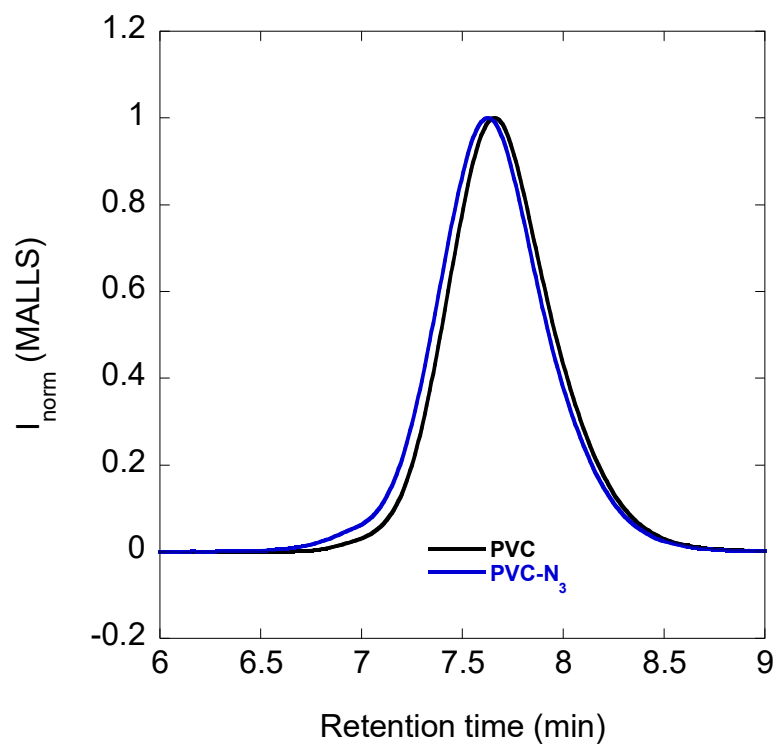
Figure S 7. GPC chromatogram (LS detector) PVC in black and PVC-N 3 in blue.
