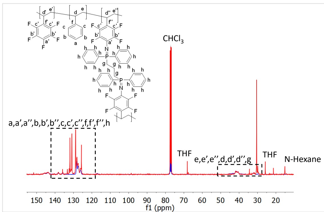
Figure S 4. ^{13}\text{C} NMR spectra of P(S-co-PFS)-SCNPs, showing the new peaks g and h related with the cross-linker.
