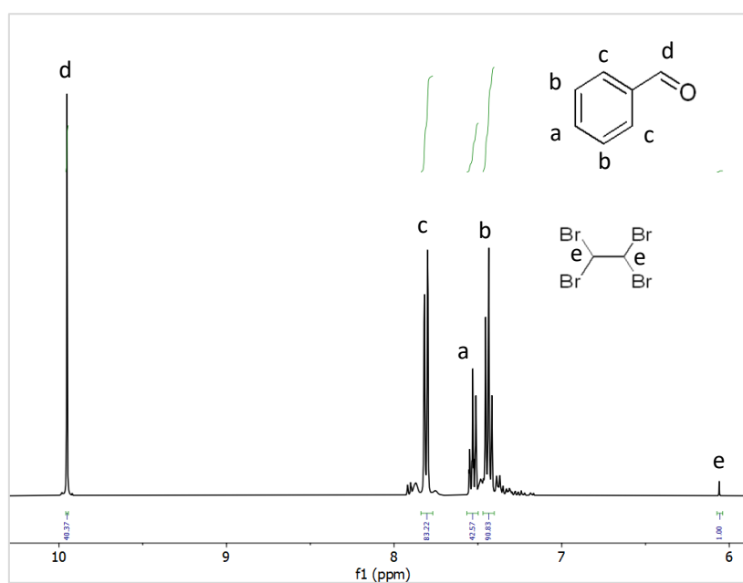
Figure 96. ^1\text{H} NMR spectra of benzaldehyde synthesized with vPVC-SCNPs/Cu(II).
