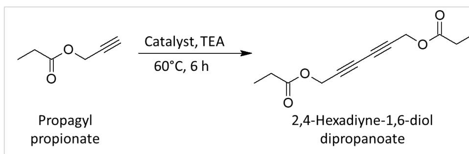
Figure 70. Synthetic scheme of 2,4-hexadiyne-1,6-diol dipropanoate.
