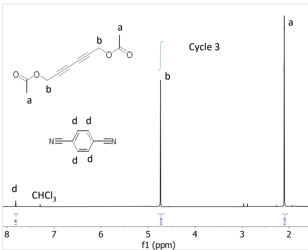
Figure S 11. ^1\text{H} NMR spectra of the hexa-2,4-diyne-1,6-diyl diacetate synthesized with vPVC-SCNPs/Cu(II) at the third cycle.
