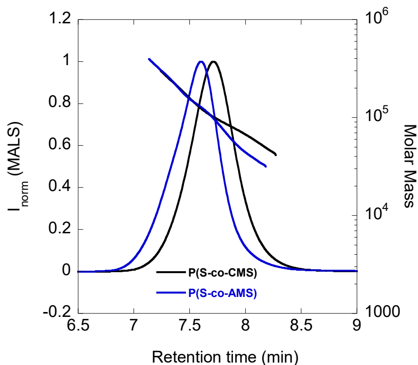
Figure 54. GPC chromatograph of P(S-co-CMS) (black) and P(S-co-AMS) (blue).
