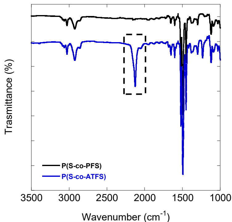
Figure 30. FTIR spectra of P(S-co-PFS) (black) and P(S-co-ATFS) (blue). In the black box is highlighted the peak that is related with the azide group.
