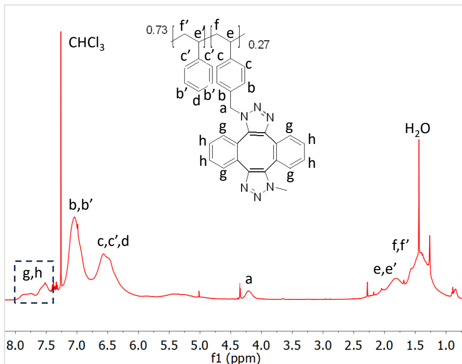
Figure 58. ^1\text{H} NMR spectrum of PS-SCNPs.
