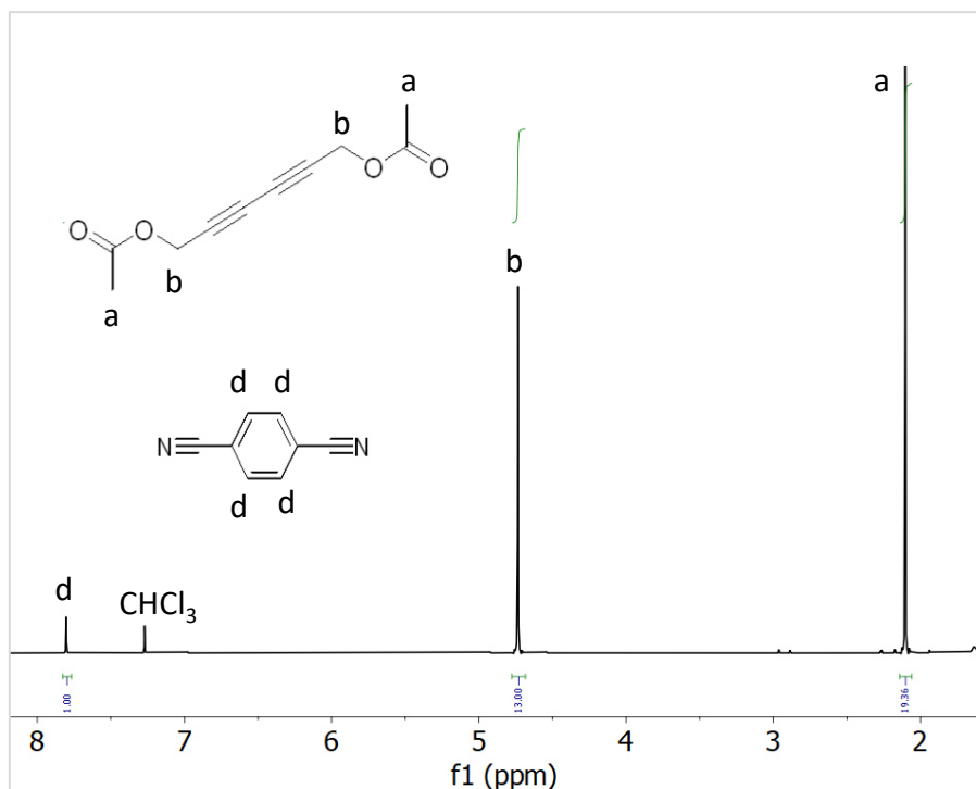
Figure 90. ^1\text{H} NMR spectra of the hexa-2,4-diyne-1,6-diyl diacetate synthesized with vPVC-SCNPs/Cu(II) at first cycle.
