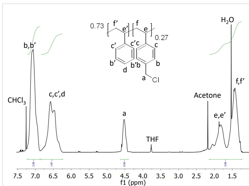
Figure 50. ^1\text{H} NMR spectrum of P(S\text{-}co\text{-}CMS) .
