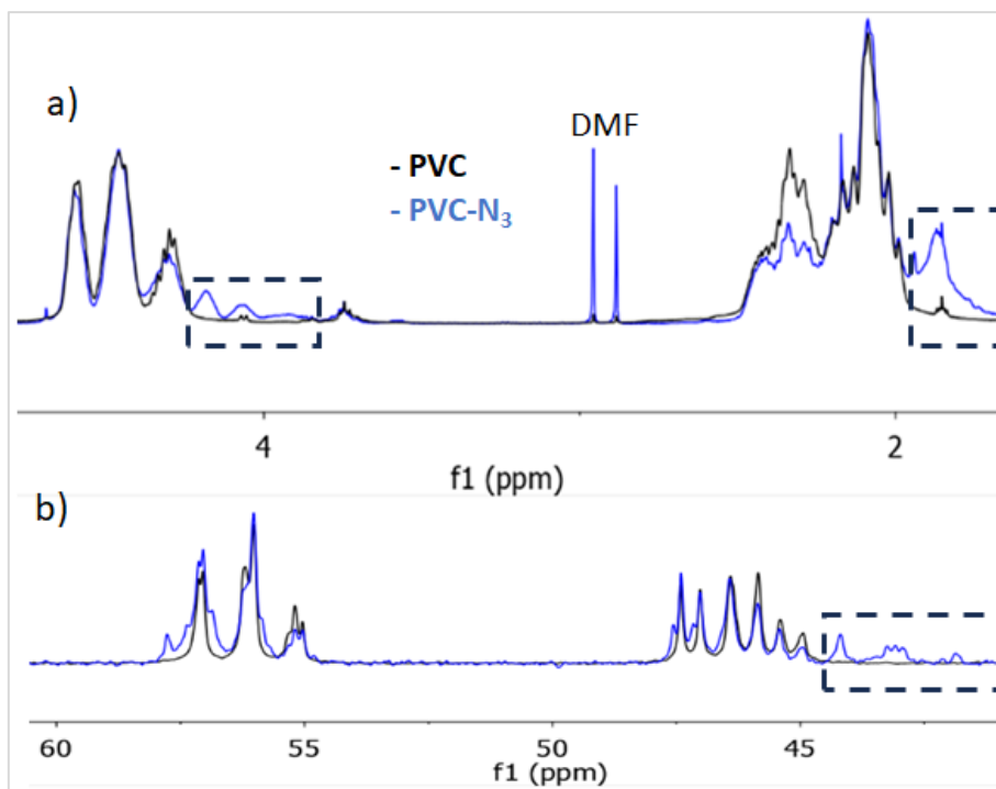
Figure 73. a) ^1\text{H} NMR and b) ^{13}\text{C} NMR spectra of PVC (black) and PVC- \text{N}_3 (blue). In the black boxes are marked the new bands associated to PVC- \text{N}_3 .
