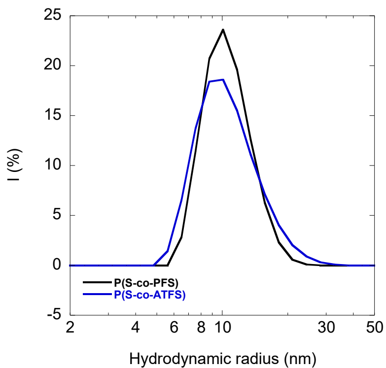
Figure S 3. DLS size distribution in THF of P(S-co-PFS) (black) and P(S-co-ATFS) (blue).
