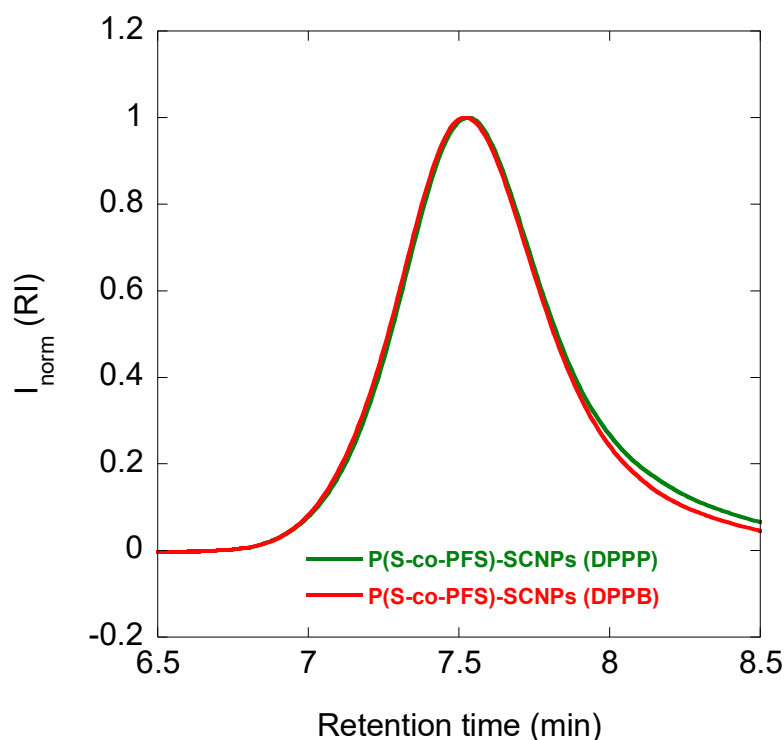
Figure 36. GPC chromatogram (RI detector) of P(S-co-PFS)-SCNPs using as cross-linker DPPP (green) and DPPB (red).
