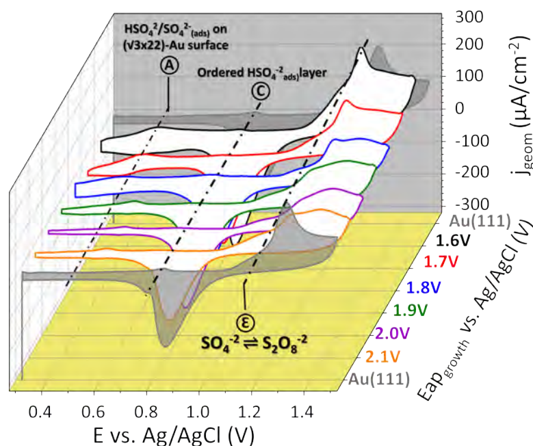
Figure 5.15: Cyclic voltammogram of Au(111) surfaces after polarization for 5 min in deaerated 0.05 M H_2SO_4 electrolyte from 0.3 to 1.5 V at a scan rate of 50 \text{ mV s}^{-1} . It is the 1 st cycle.
