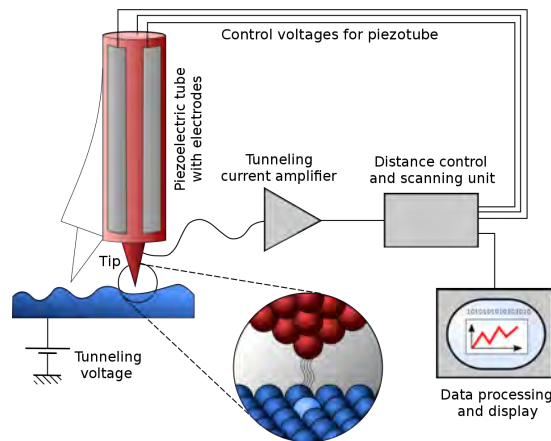
Figure 3.4: Schematic representation of the working principle of scanning tunneling microscopy (STM) obtained from [116].
