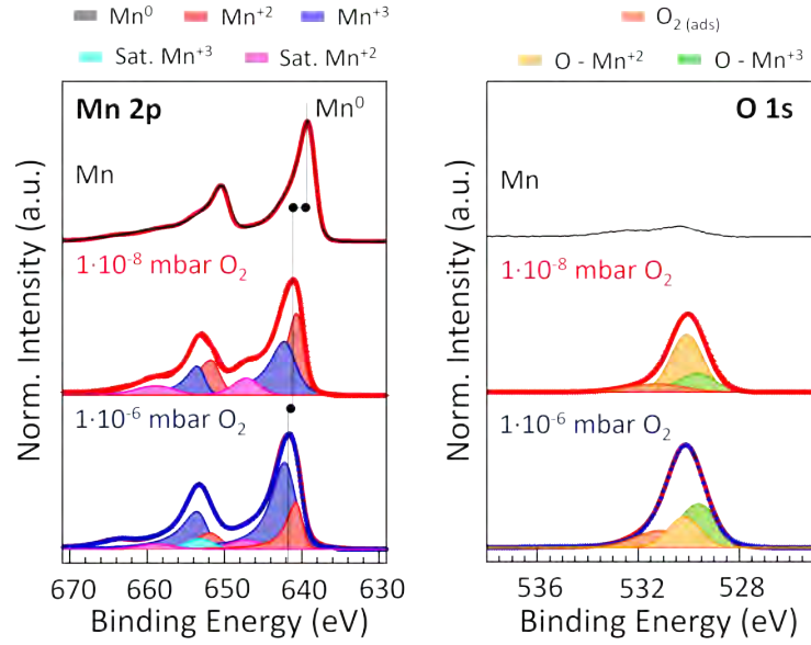
Figure 6.12: XPS spectra and fitting components at the energies of (left) Mn 2p and (right) O 1s core levels for different manganese-based oxides grown at room temperature under different oxygen partial pressure as well as oxidizing agent: (black) in absence of oxidizing agent, (red) under 10^{-8} mbar and (blue) 10^{-6} mbar molecular oxygen partial pressure.
