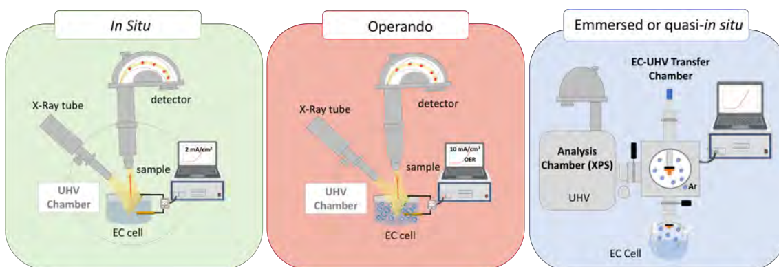
Figure 4.2: Schematic representation of, from left to right, in situ , operando, and emersed or quasi- in situ approaches.
