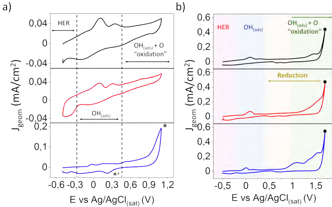
Figure 6.20: Cyclic voltammograms obtained in an Ar-purged 0.05 M NaOH at 50 mV/s in two different potential ranges: a) from OCP to 1.1 V and b) from OCP to 1.7 V for different samples, (black) Mn/Au(111), (blue) MnO/Au(111) and (red) Mn_3O_4 /Au(111).
