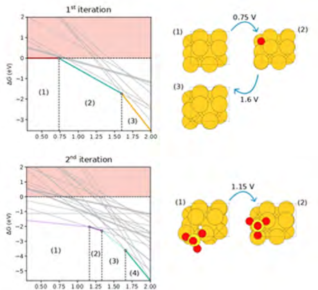
Figure 5.16: ESPD slice depicting the pH 1.3 on a gold surface. The panels unveil slices obtained through two distinct methodological iterations, each advancing the depiction of surface configurations. Accompanying each iteration are the atomic arrangement associated with various stability domains.
